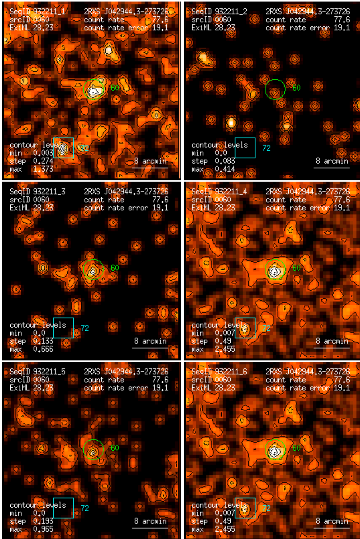
Figure 60: RASS 932211: detection 0060: band rate images, Gaussian filter: (1) PSPC channels 11 – 41, (2) 52 – 90, (3) 91 – 201, (4) 11 – 235, (5) 52 – 201, (6) 11 – 201. Broad band rates in counts/ks. Band rate contour levels in counts/ks/arcmin 2 .
