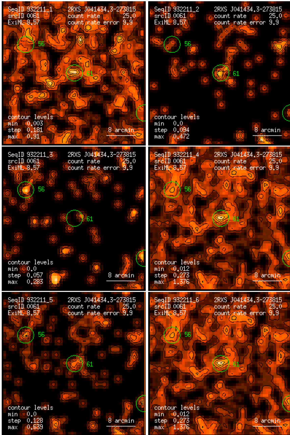
Figure 61: RASS 932211: detection 0061: band rate images, Gaussian filter: (1) PSPC channels 11 – 41, (2) 52 – 90, (3) 91 – 201, (4) 11 – 235, (5) 52 – 201, (6) 11 – 201. Broad band rates in counts/ks. Band rate contour levels in counts/ks/arcmin 2 .
