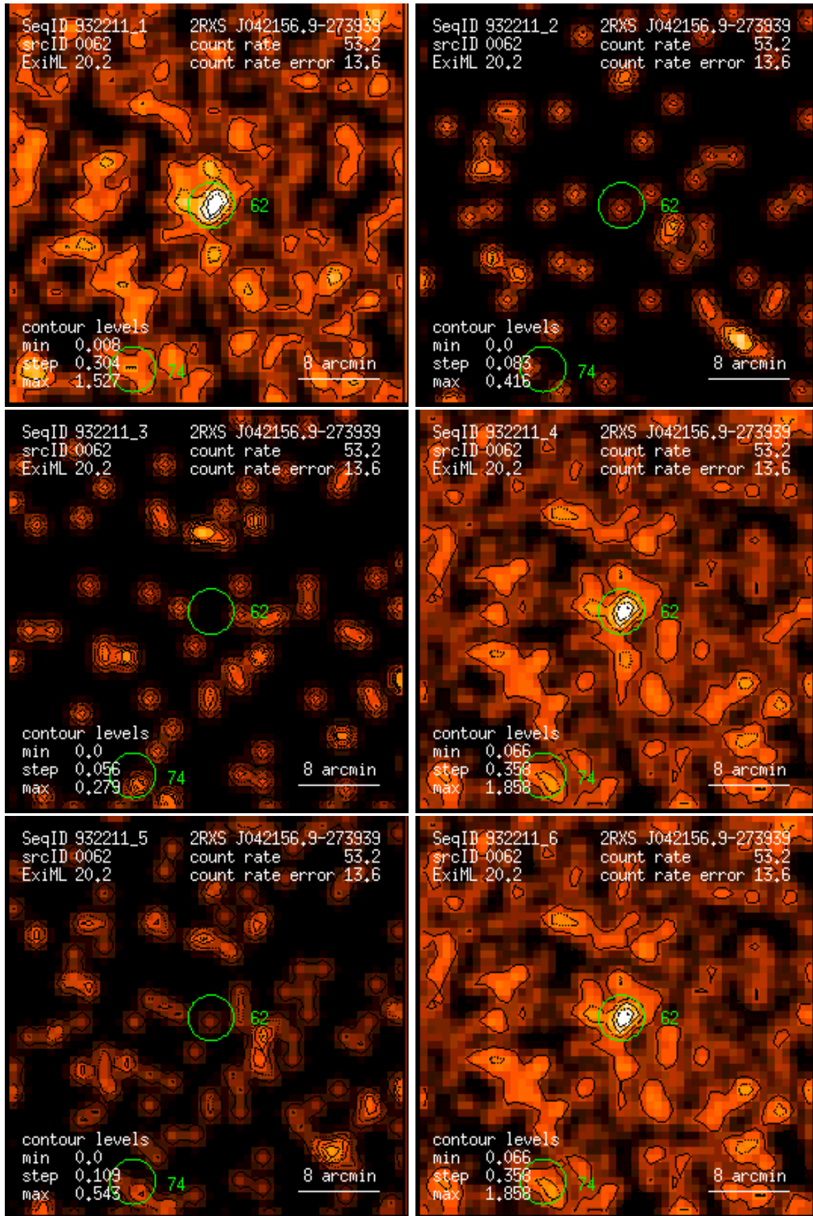
Figure 62: RASS 932211: detection 0062: band rate images, Gaussian filter: (1) PSPC channels 11 – 41, (2) 52 – 90, (3) 91 – 201, (4) 11 – 235, (5) 52 – 201, (6) 11 – 201. Broad band rates in counts/ks. Band rate contour levels in counts/ks/arcmin 2 .
