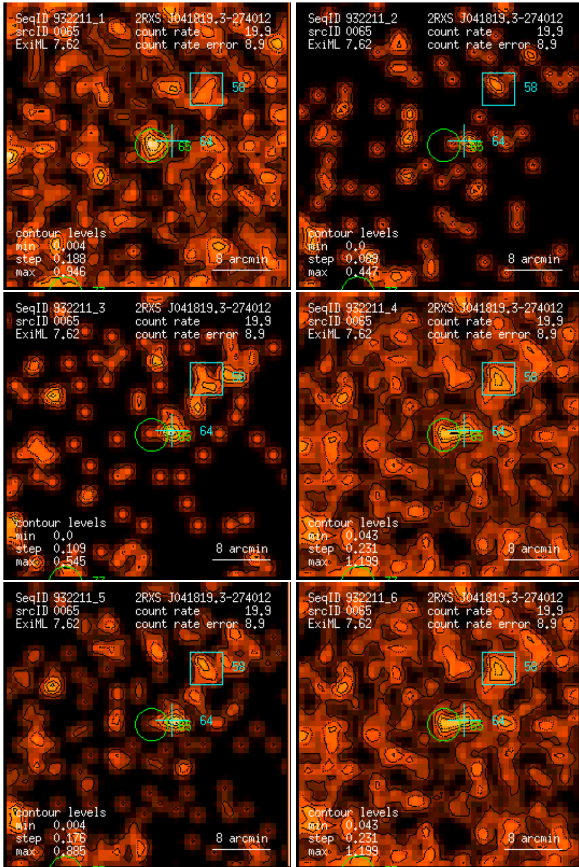
Figure 65: RASS 932211: detection 0065: band rate images, Gaussian filter: (1) PSPC channels 11 – 41, (2) 52 – 90, (3) 91 – 201, (4) 11 – 235, (5) 52 – 201, (6) 11 – 201. Broad band rates in counts/ks. Band rate contour levels in counts/ks/arcmin 2 .
