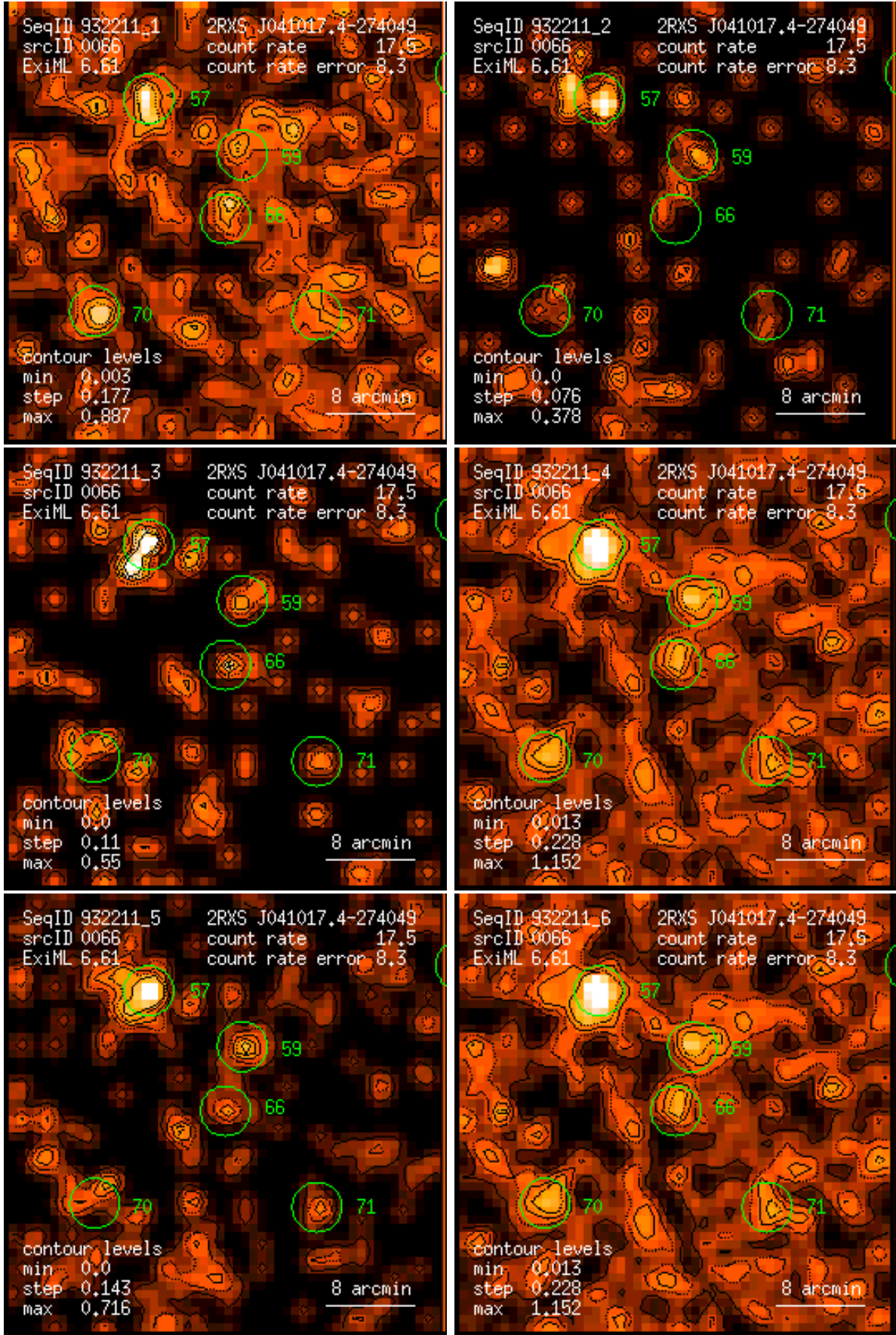
Figure 66: RASS 932211: detection 0066: band rate images, Gaussian filter: (1) PSPC channels 11 – 41, (2) 52 – 90, (3) 91 – 201, (4) 11 – 235, (5) 52 – 201, (6) 11 – 201. Broad band rates in counts/ks. Band rate contour levels in counts/ks/arcmin 2 .
