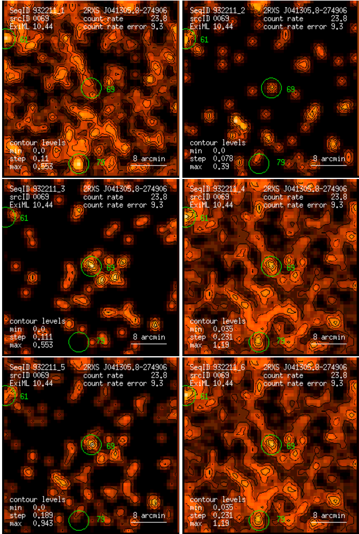
Figure 69: RASS 932211: detection 0069: band rate images, Gaussian filter: (1) PSPC channels 11 – 41, (2) 52 – 90, (3) 91 – 201, (4) 11 – 235, (5) 52 – 201, (6) 11 – 201. Broad band rates in counts/ks. Band rate contour levels in counts/ks/arcmin 2 .
