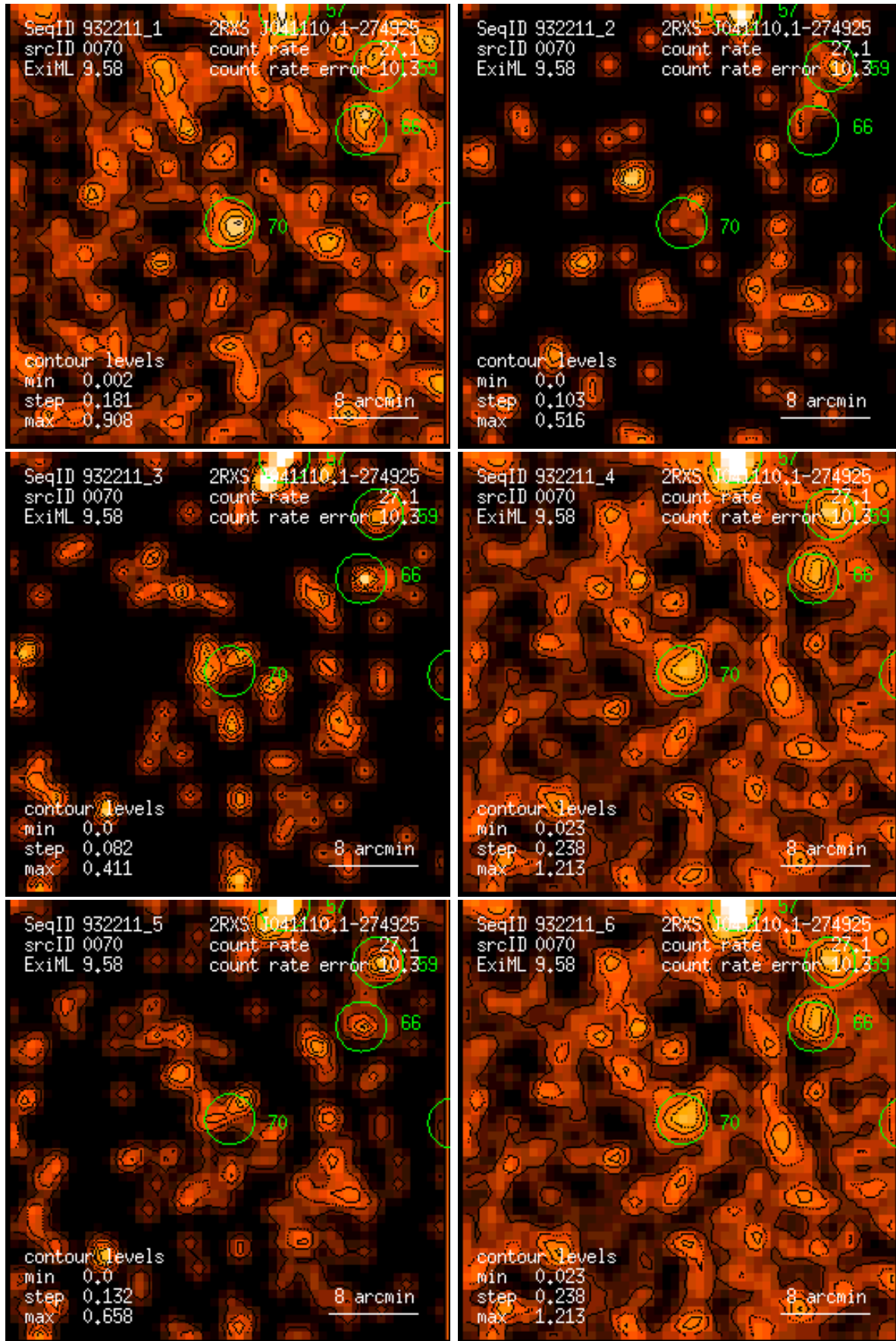
Figure 70: RASS 932211: detection 0070: band rate images, Gaussian filter: (1) PSPC channels 11 – 41, (2) 52 – 90, (3) 91 – 201, (4) 11 – 235, (5) 52 – 201, (6) 11 – 201. Broad band rates in counts/ks. Band rate contour levels in counts/ks/arcmin 2 .
