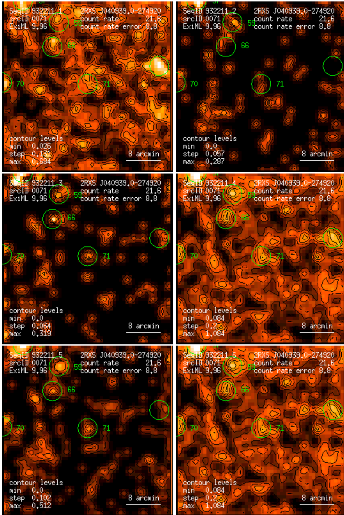
Figure 71: RASS 932211: detection 0071: band rate images, Gaussian filter: (1) PSPC channels 11 – 41, (2) 52 – 90, (3) 91 – 201, (4) 11 – 235, (5) 52 – 201, (6) 11 – 201. Broad band rates in counts/ks. Band rate contour levels in counts/ks/arcmin 2 .
