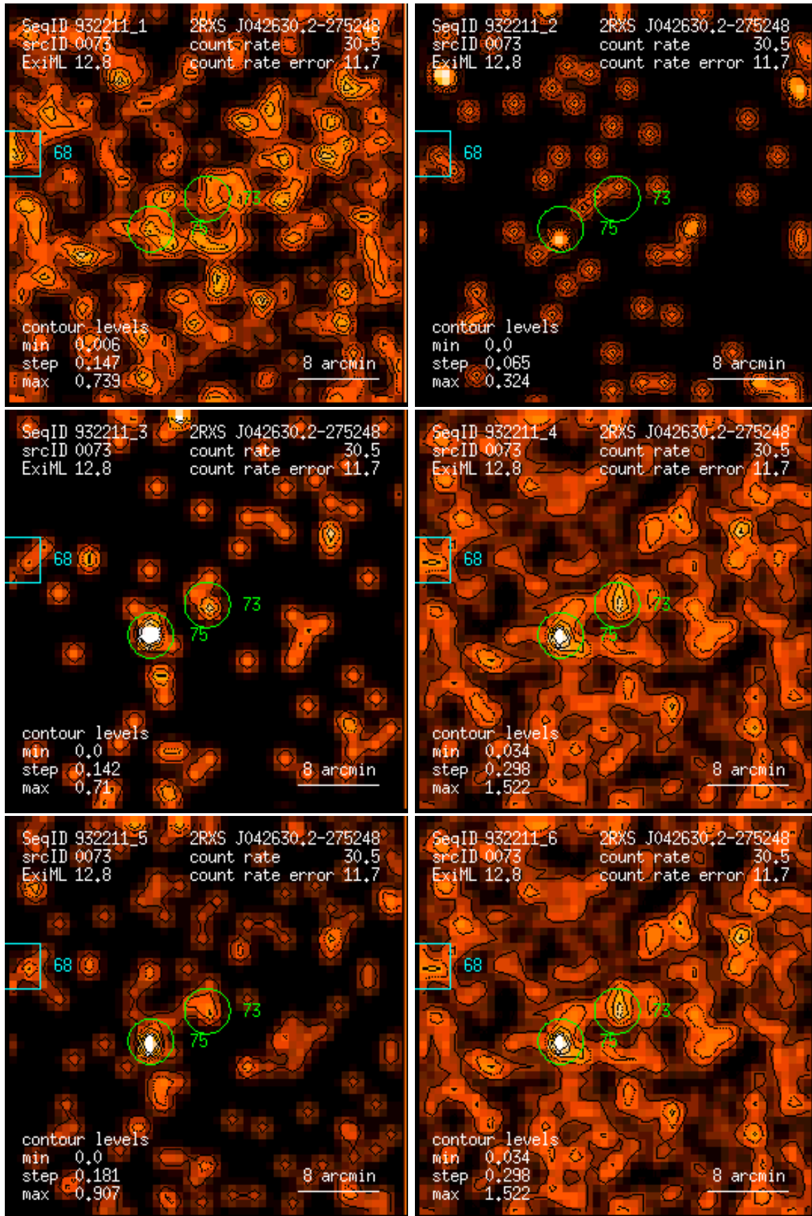
Figure 73: RASS 932211: detection 0073: band rate images, Gaussian filter: (1) PSPC channels 11 – 41, (2) 52 – 90, (3) 91 – 201, (4) 11 – 235, (5) 52 – 201, (6) 11 – 201. Broad band rates in counts/ks. Band rate contour levels in counts/ks/arcmin 2 .
