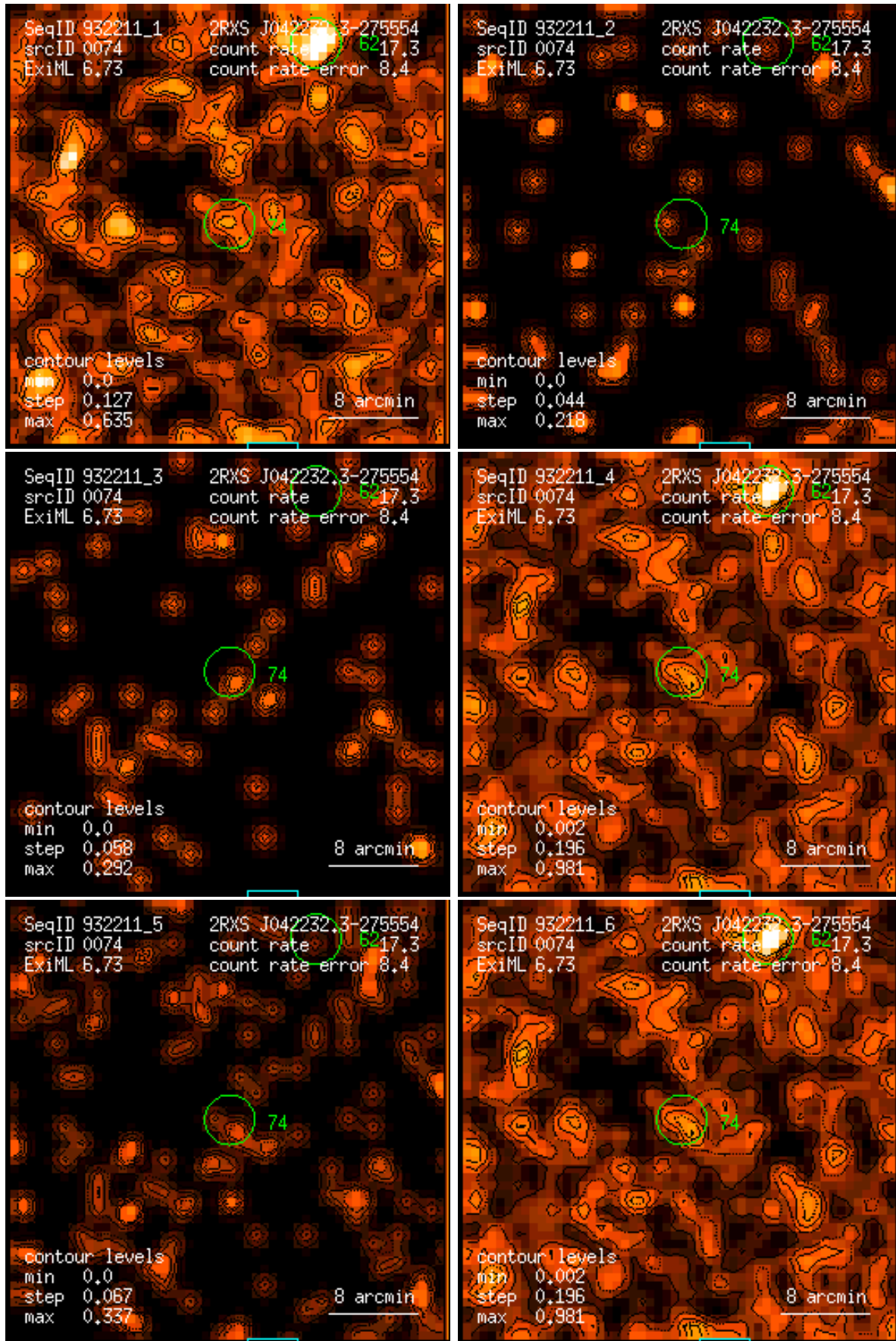
Figure 74: RASS 932211: detection 0074: band rate images, Gaussian filter: (1) PSPC channels 11 – 41, (2) 52 – 90, (3) 91 – 201, (4) 11 – 235, (5) 52 – 201, (6) 11 – 201. Broad band rates in counts/ks. Band rate contour levels in counts/ks/arcmin 2 .
