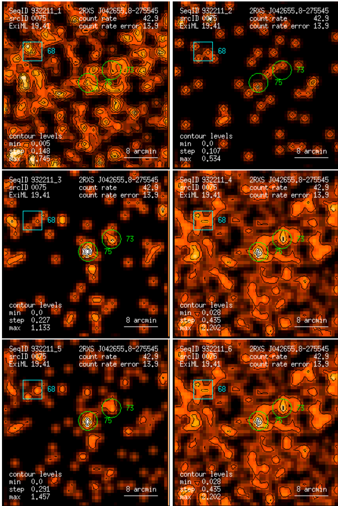
Figure 75: RASS 932211: detection 0075: band rate images, Gaussian filter: (1) PSPC channels 11 – 41, (2) 52 – 90, (3) 91 – 201, (4) 11 – 235, (5) 52 – 201, (6) 11 – 201. Broad band rates in counts/ks. Band rate contour levels in counts/ks/arcmin 2 .
