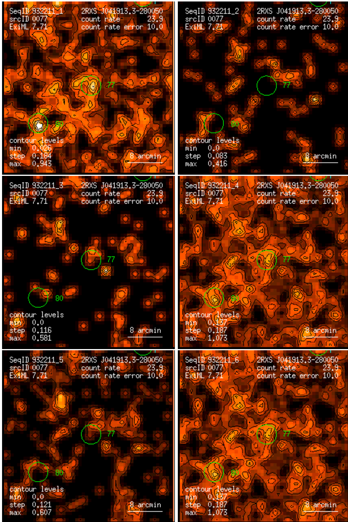
Figure 77: RASS 932211: detection 0077: band rate images, Gaussian filter: (1) PSPC channels 11 – 41, (2) 52 – 90, (3) 91 – 201, (4) 11 – 235, (5) 52 – 201, (6) 11 – 201. Broad band rates in counts/ks. Band rate contour levels in counts/ks/arcmin 2 .
