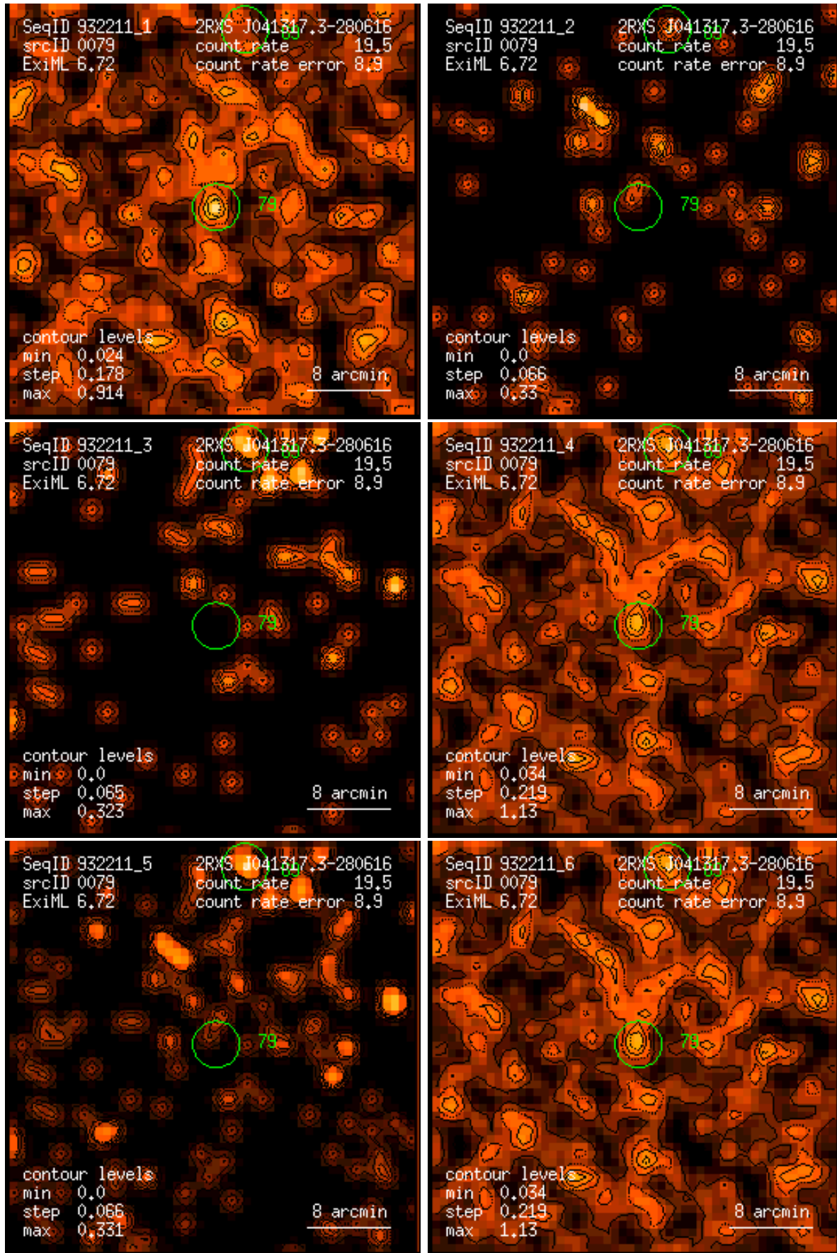
Figure 79: RASS 932211: detection 0079: band rate images, Gaussian filter: (1) PSPC channels 11 – 41, (2) 52 – 90, (3) 91 – 201, (4) 11 – 235, (5) 52 – 201, (6) 11 – 201. Broad band rates in counts/ks. Band rate contour levels in counts/ks/arcmin 2 .
