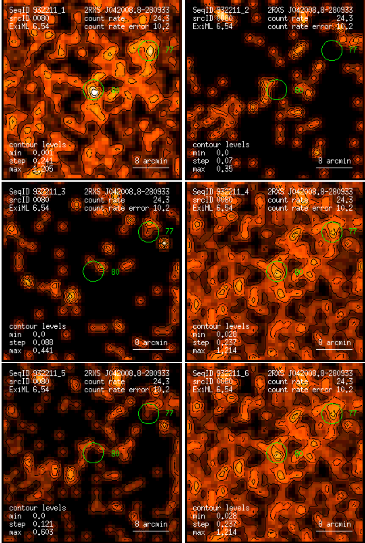
Figure 80: RASS 932211: detection 0080: band rate images, Gaussian filter: (1) PSPC channels 11 – 41, (2) 52 – 90, (3) 91 – 201, (4) 11 – 235, (5) 52 – 201, (6) 11 – 201. Broad band rates in counts/ks. Band rate contour levels in counts/ks/arcmin 2 .
