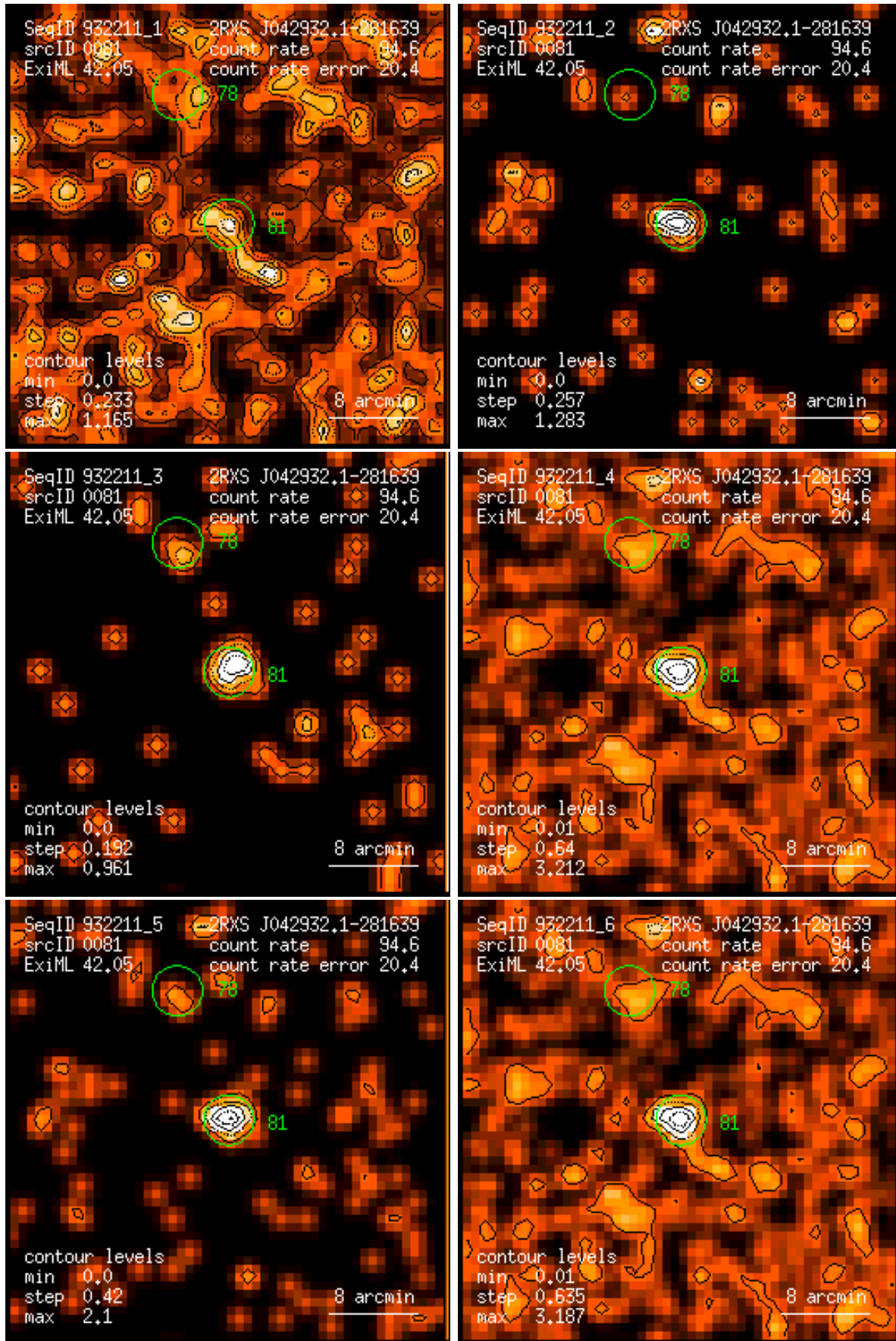
Figure 81: RASS 932211: detection 0081: band rate images, Gaussian filter: (1) PSPC channels 11 – 41, (2) 52 – 90, (3) 91 – 201, (4) 11 – 235, (5) 52 – 201, (6) 11 – 201. Broad band rates in counts/ks. Band rate contour levels in counts/ks/arcmin 2 .
