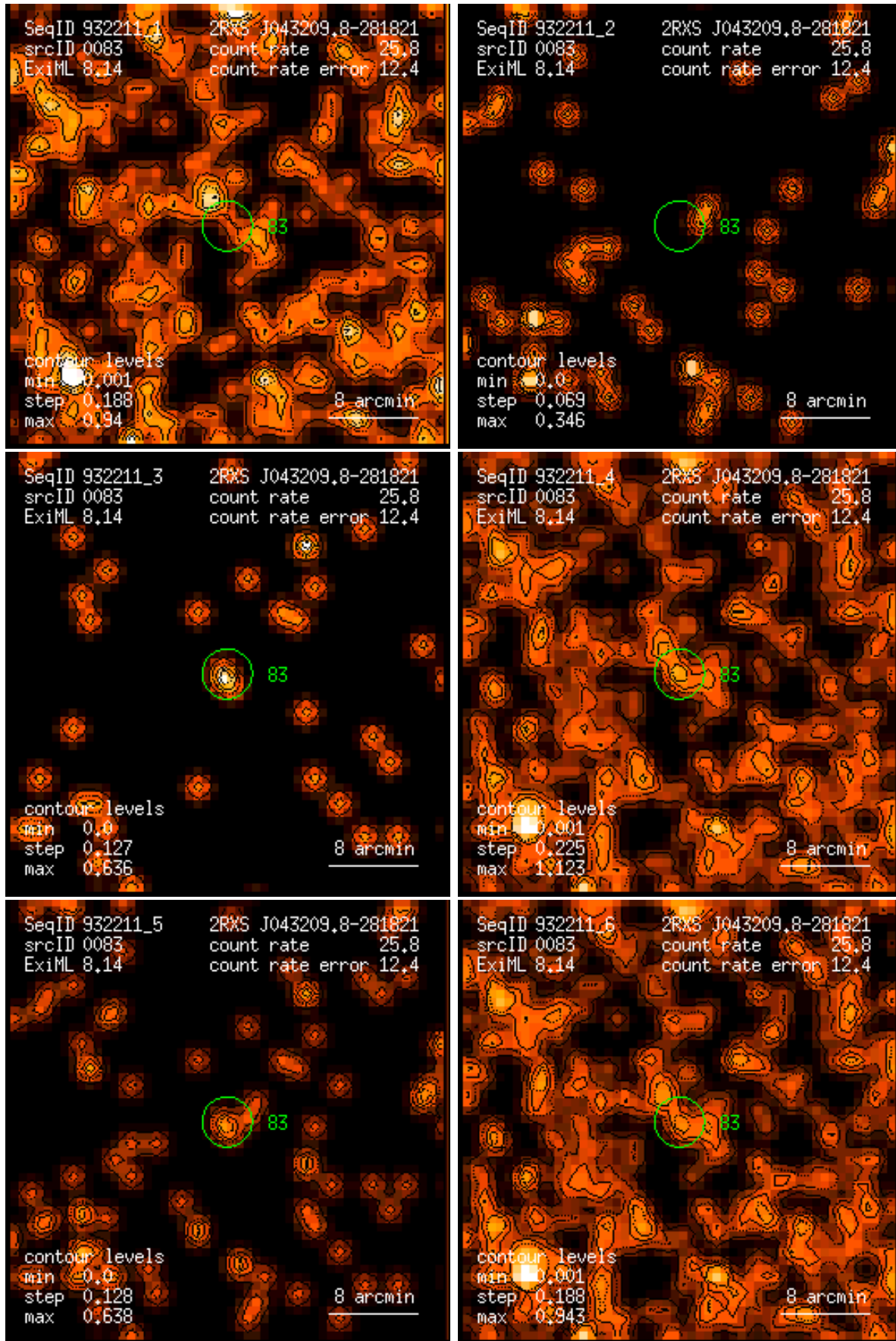
Figure 83: RASS 932211: detection 0083: band rate images, Gaussian filter: (1) PSPC channels 11 – 41, (2) 52 – 90, (3) 91 – 201, (4) 11 – 235, (5) 52 – 201, (6) 11 – 201. Broad band rates in counts/ks. Band rate contour levels in counts/ks/arcmin 2 .
