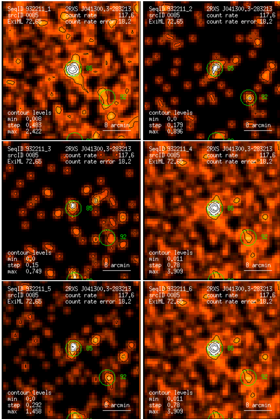
Figure 85: RASS 932211: detection 0085: band rate images, Gaussian filter: (1) PSPC channels 11 – 41, (2) 52 – 90, (3) 91 – 201, (4) 11 – 235, (5) 52 – 201, (6) 11 – 201. Broad band rates in counts/ks. Band rate contour levels in counts/ks/arcmin 2 .
