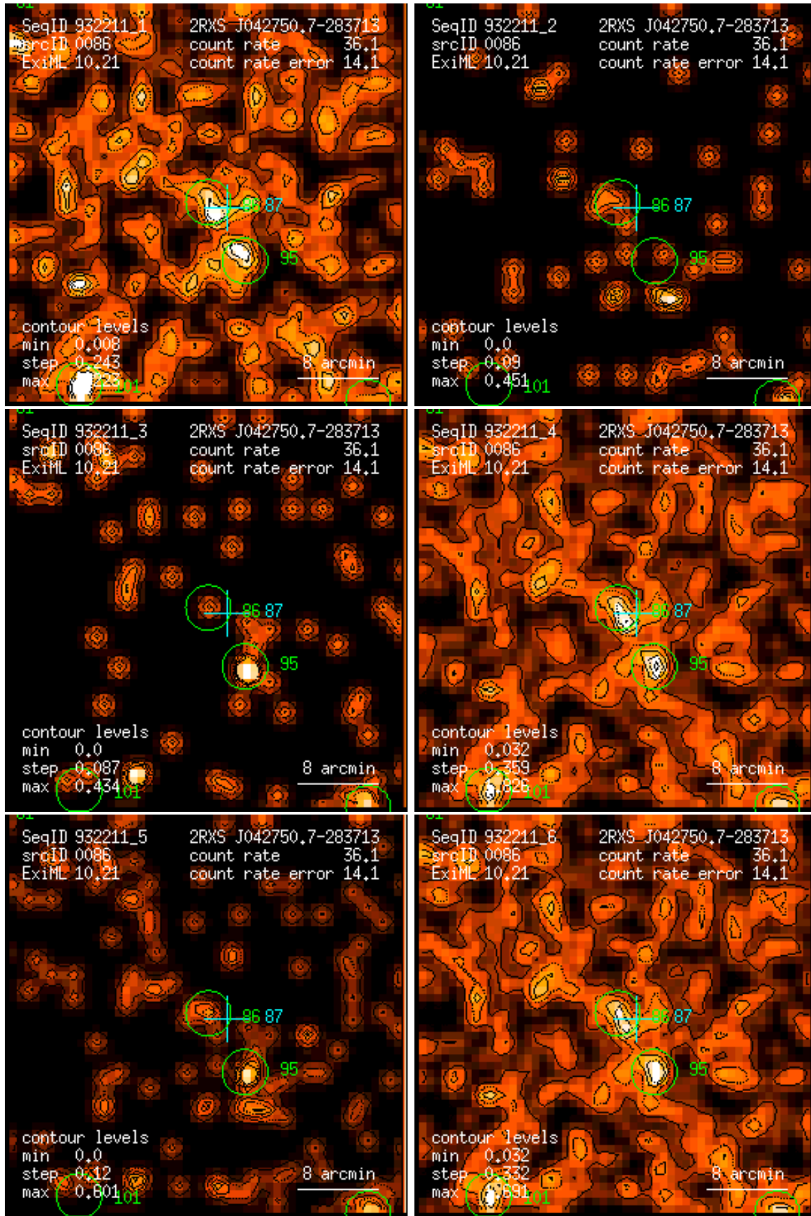
Figure 86: RASS 932211: detection 0086: band rate images, Gaussian filter: (1) PSPC channels 11 – 41, (2) 52 – 90, (3) 91 – 201, (4) 11 – 235, (5) 52 – 201, (6) 11 – 201. Broad band rates in counts/ks. Band rate contour levels in counts/ks/arcmin 2 .
