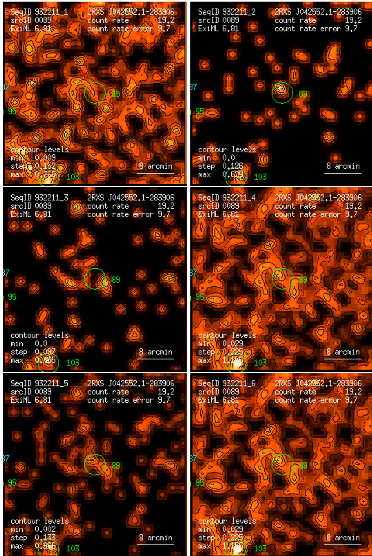
Figure 89: RASS 932211: detection 0089: band rate images, Gaussian filter: (1) PSPC channels 11 – 41, (2) 52 – 90, (3) 91 – 201, (4) 11 – 235, (5) 52 – 201, (6) 11 – 201. Broad band rates in counts/ks. Band rate contour levels in counts/ks/arcmin 2 .
