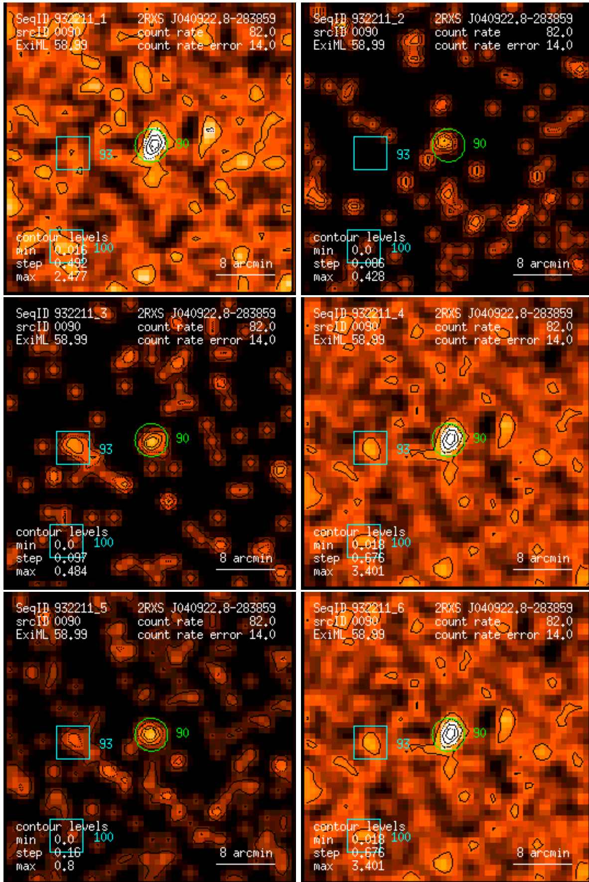
Figure 90: RASS 932211: detection 0090: band rate images, Gaussian filter: (1) PSPC channels 11 – 41, (2) 52 – 90, (3) 91 – 201, (4) 11 – 235, (5) 52 – 201, (6) 11 – 201. Broad band rates in counts/ks. Band rate contour levels in counts/ks/arcmin 2 .
