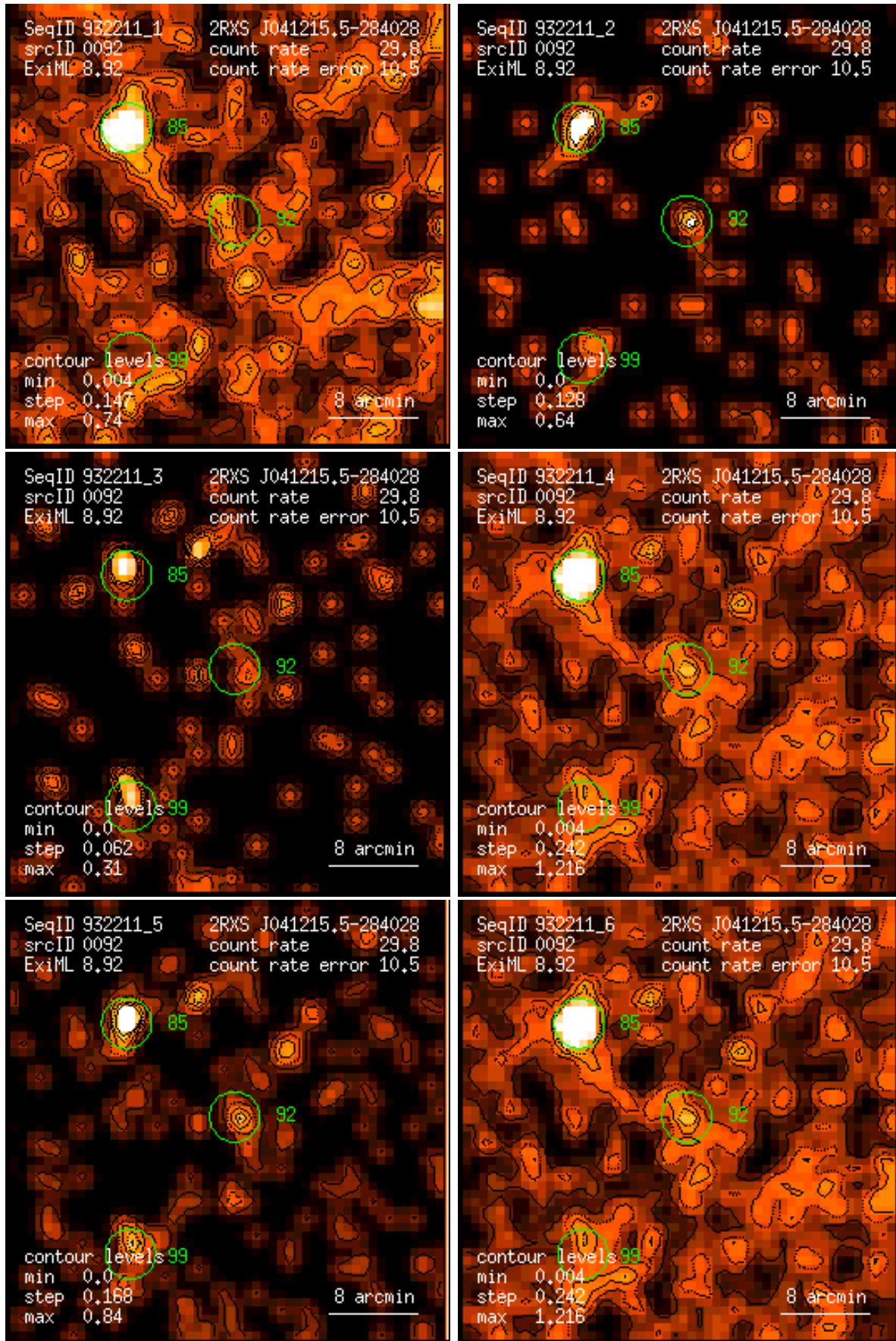
Figure 92: RASS 932211: detection 0092: band rate images, Gaussian filter: (1) PSPC channels 11 – 41, (2) 52 – 90, (3) 91 – 201, (4) 11 – 235, (5) 52 – 201, (6) 11 – 201. Broad band rates in counts/ks. Band rate contour levels in counts/ks/arcmin 2 .
