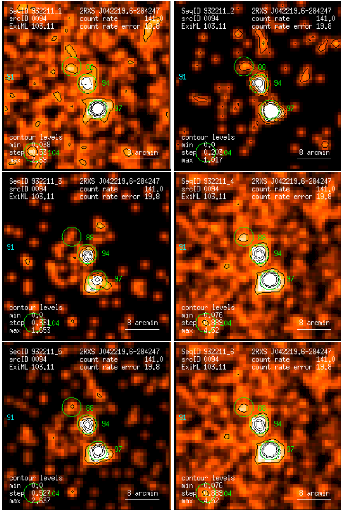
Figure 94: RASS 932211: detection 0094: band rate images, Gaussian filter: (1) PSPC channels 11 – 41, (2) 52 – 90, (3) 91 – 201, (4) 11 – 235, (5) 52 – 201, (6) 11 – 201. Broad band rates in counts/ks. Band rate contour levels in counts/ks/arcmin 2 .
