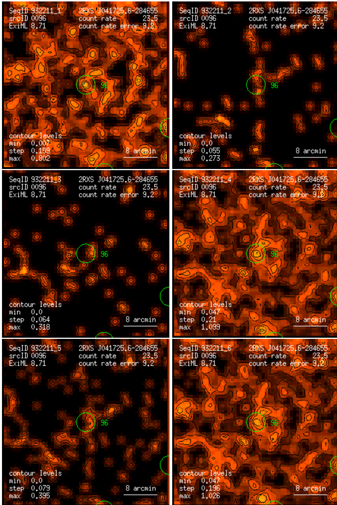
Figure 96: RASS 932211: detection 0096: band rate images, Gaussian filter: (1) PSPC channels 11 – 41, (2) 52 – 90, (3) 91 – 201, (4) 11 – 235, (5) 52 – 201, (6) 11 – 201. Broad band rates in counts/ks. Band rate contour levels in counts/ks/arcmin 2 .
