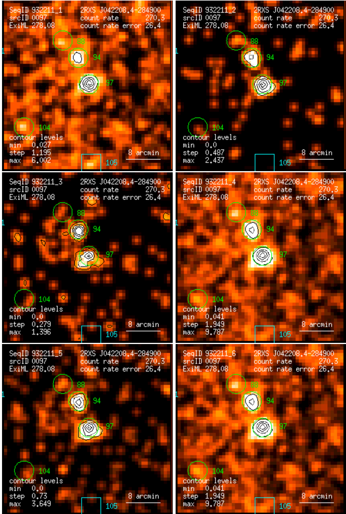
Figure 97: RASS 932211: detection 0097: band rate images, Gaussian filter: (1) PSPC channels 11 – 41, (2) 52 – 90, (3) 91 – 201, (4) 11 – 235, (5) 52 – 201, (6) 11 – 201. Broad band rates in counts/ks. Band rate contour levels in counts/ks/arcmin 2 .
