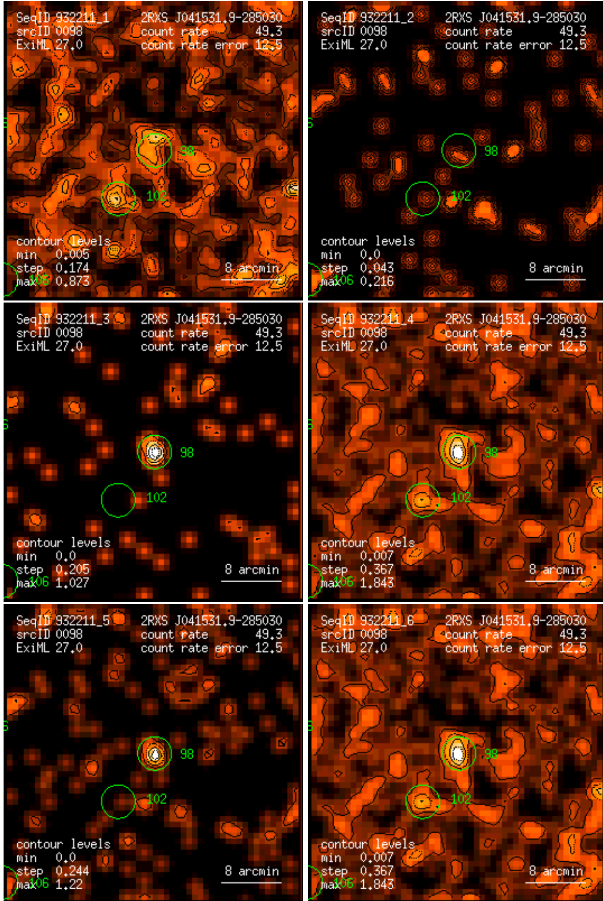
Figure 98: RASS 932211: detection 0098: band rate images, Gaussian filter: (1) PSPC channels 11 – 41, (2) 52 – 90, (3) 91 – 201, (4) 11 – 235, (5) 52 – 201, (6) 11 – 201. Broad band rates in counts/ks. Band rate contour levels in counts/ks/arcmin 2 .
