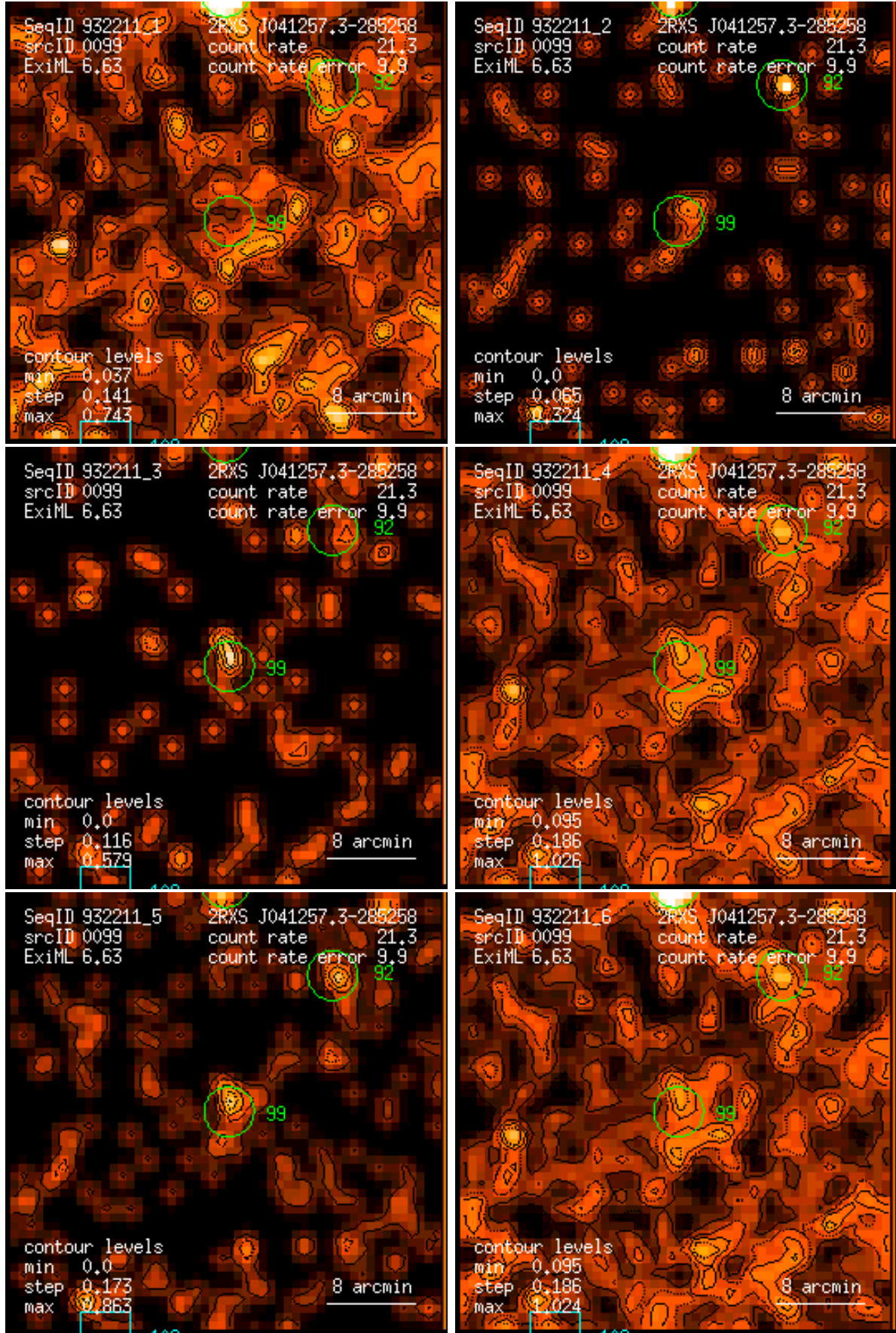
Figure 99: RASS 932211: detection 0099: band rate images, Gaussian filter: (1) PSPC channels 11 – 41, (2) 52 – 90, (3) 91 – 201, (4) 11 – 235, (5) 52 – 201, (6) 11 – 201. Broad band rates in counts/ks. Band rate contour levels in counts/ks/arcmin 2 .
