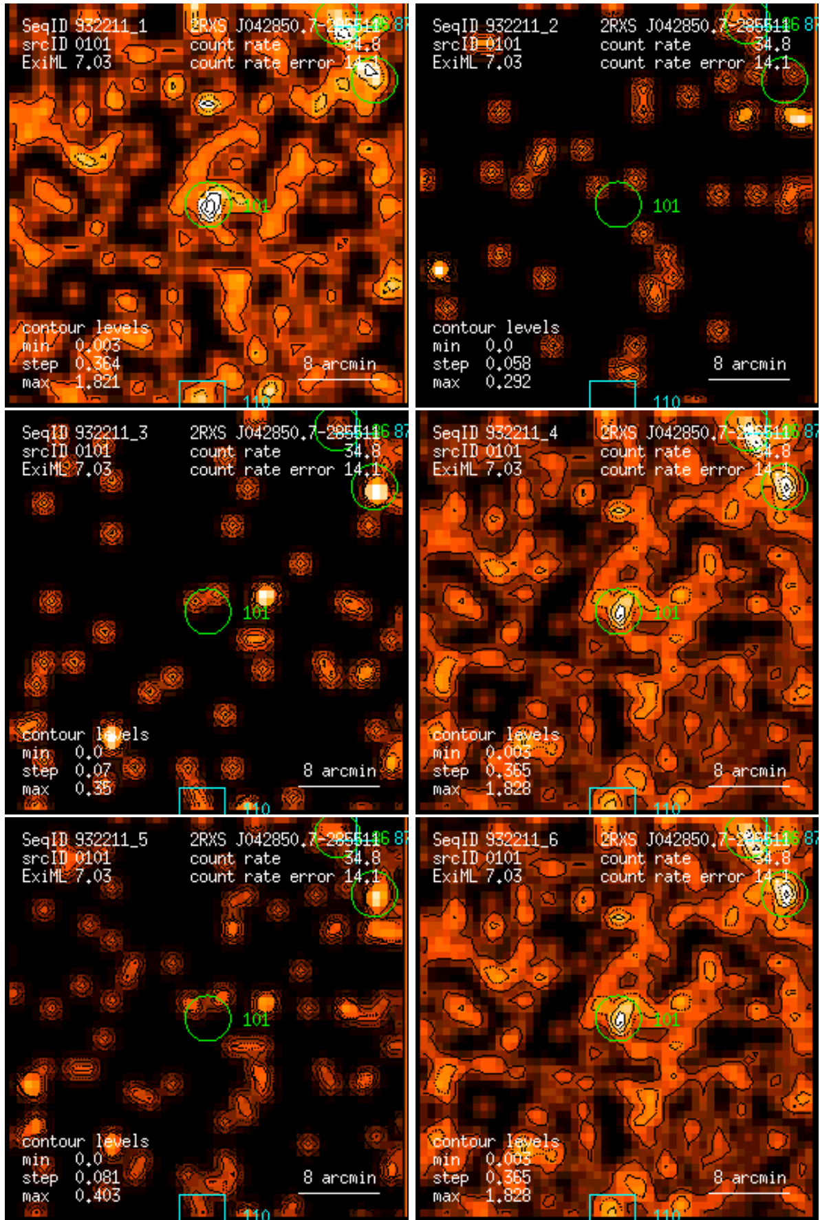
Figure 101: RASS 932211: detection 0101: band rate images, Gaussian filter: (1) PSPC channels 11 – 41, (2) 52 – 90, (3) 91 – 201, (4) 11 – 235, (5) 52 – 201, (6) 11 – 201. Broad band rates in counts/ks. Band rate contour levels in counts/ks/arcmin 2 .
