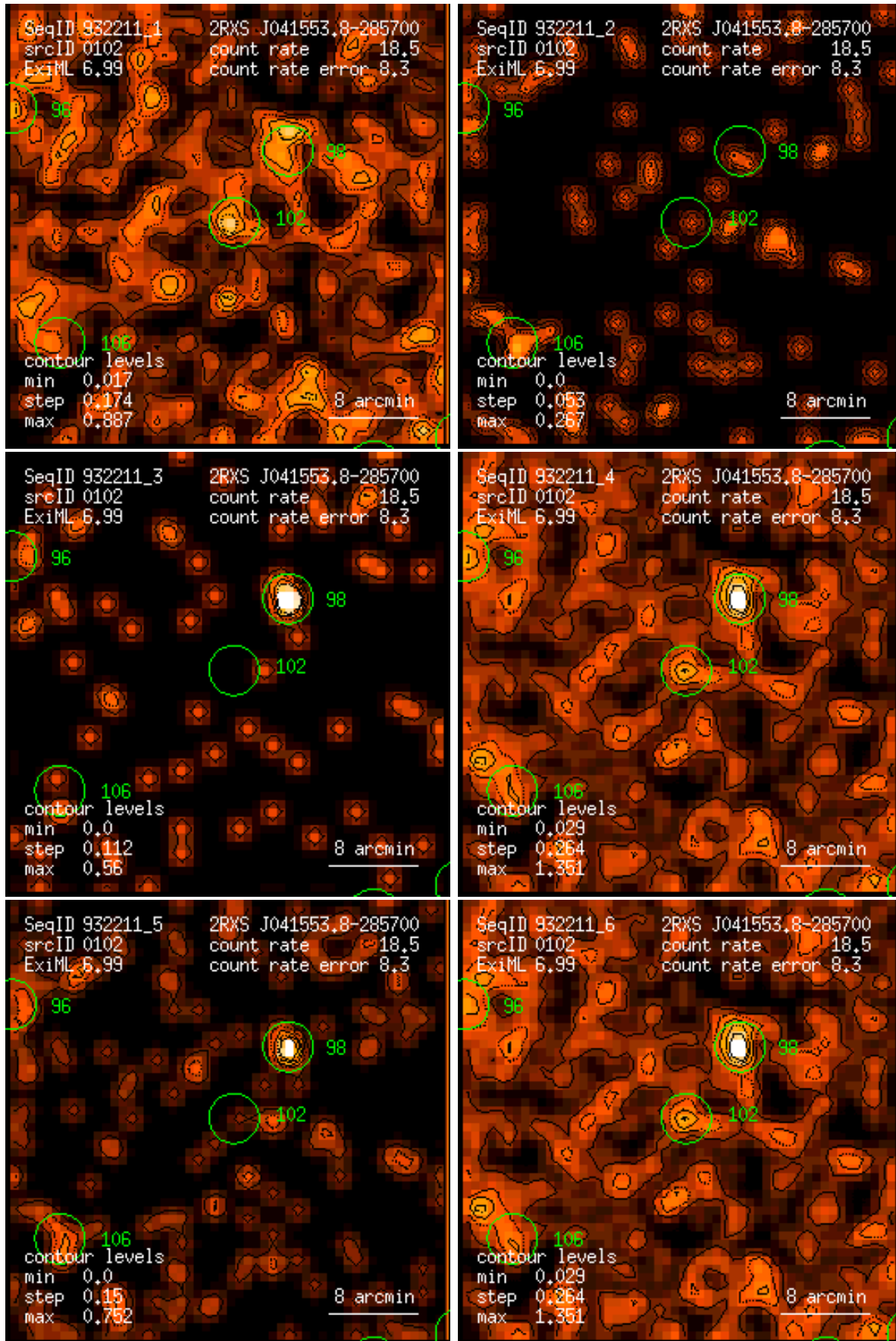
Figure 102: RASS 932211: detection 0102: band rate images, Gaussian filter: (1) PSPC channels 11 – 41, (2) 52 – 90, (3) 91 – 201, (4) 11 – 235, (5) 52 – 201, (6) 11 – 201. Broad band rates in counts/ks. Band rate contour levels in counts/ks/arcmin 2 .
