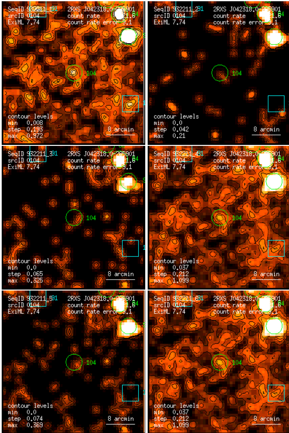
Figure 104: RASS 932211: detection 0104: band rate images, Gaussian filter: (1) PSPC channels 11 – 41, (2) 52 – 90, (3) 91 – 201, (4) 11 – 235, (5) 52 – 201, (6) 11 – 201. Broad band rates in counts/ks. Band rate contour levels in counts/ks/arcmin 2 .
