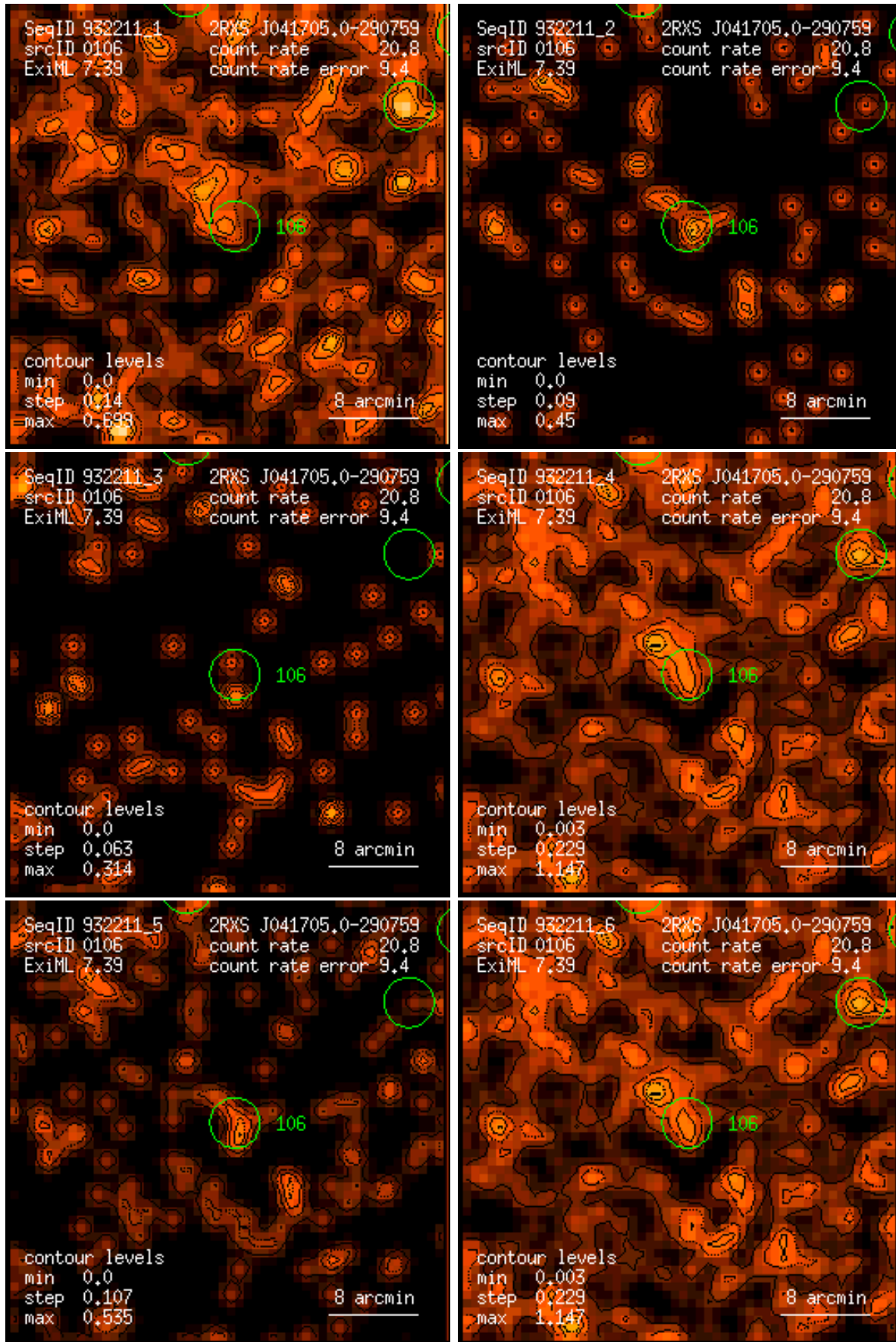
Figure 106: RASS 932211: detection 0106: band rate images, Gaussian filter: (1) PSPC channels 11 – 41, (2) 52 – 90, (3) 91 – 201, (4) 11 – 235, (5) 52 – 201, (6) 11 – 201. Broad band rates in counts/ks. Band rate contour levels in counts/ks/arcmin 2 .
