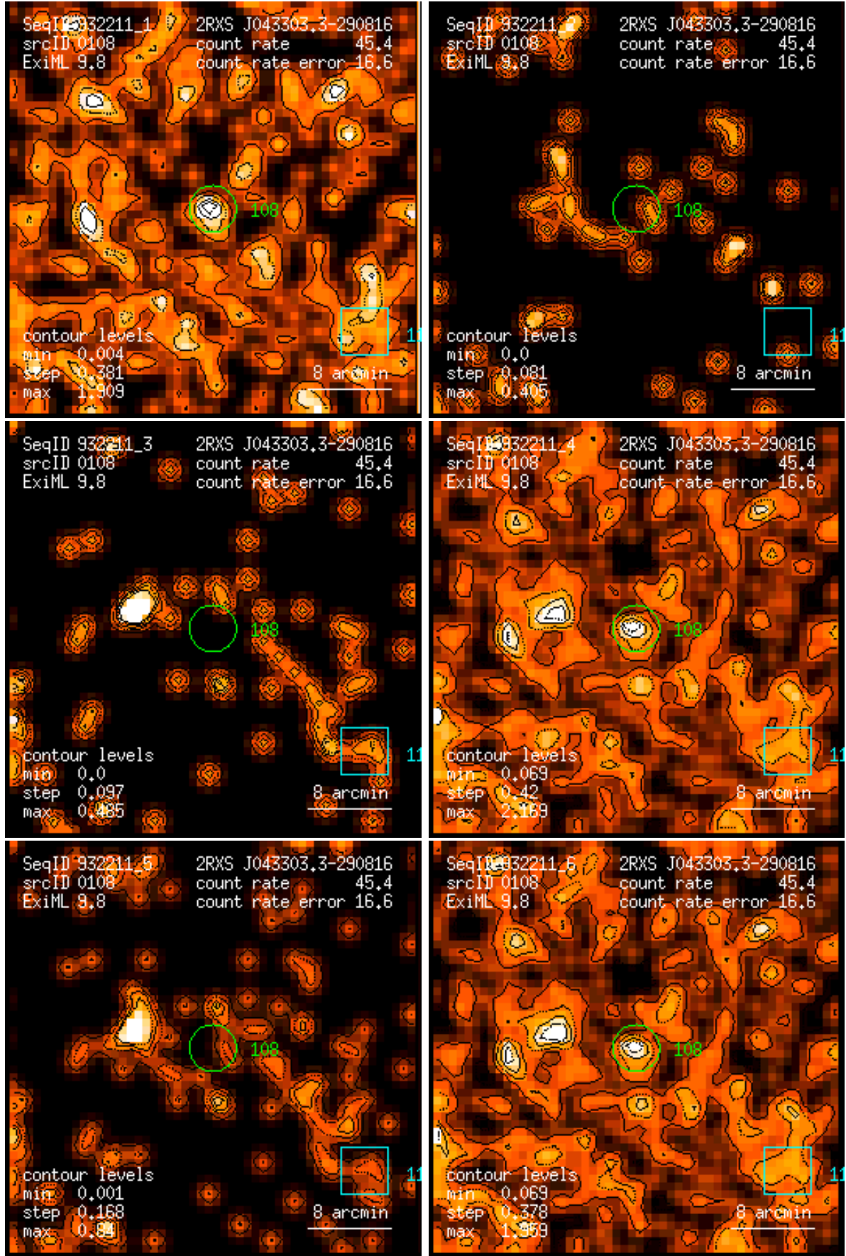
Figure 108: RASS 932211: detection 0108: band rate images, Gaussian filter: (1) PSPC channels 11 – 41, (2) 52 – 90, (3) 91 – 201, (4) 11 – 235, (5) 52 – 201, (6) 11 – 201. Broad band rates in counts/ks. Band rate contour levels in counts/ks/arcmin 2 .
