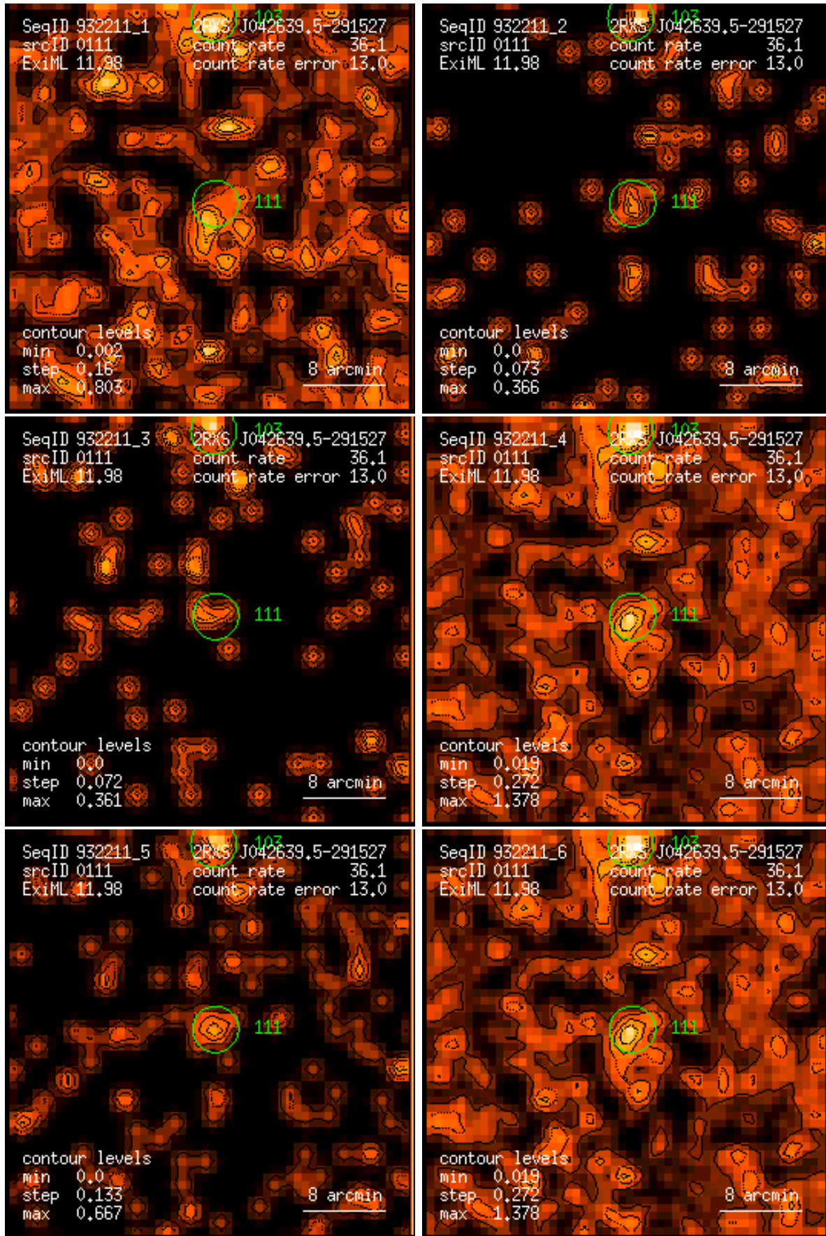
Figure 111: RASS 932211: detection 0111: band rate images, Gaussian filter: (1) PSPC channels 11 – 41, (2) 52 – 90, (3) 91 – 201, (4) 11 – 235, (5) 52 – 201, (6) 11 – 201. Broad band rates in counts/ks. Band rate contour levels in counts/ks/arcmin 2 .
