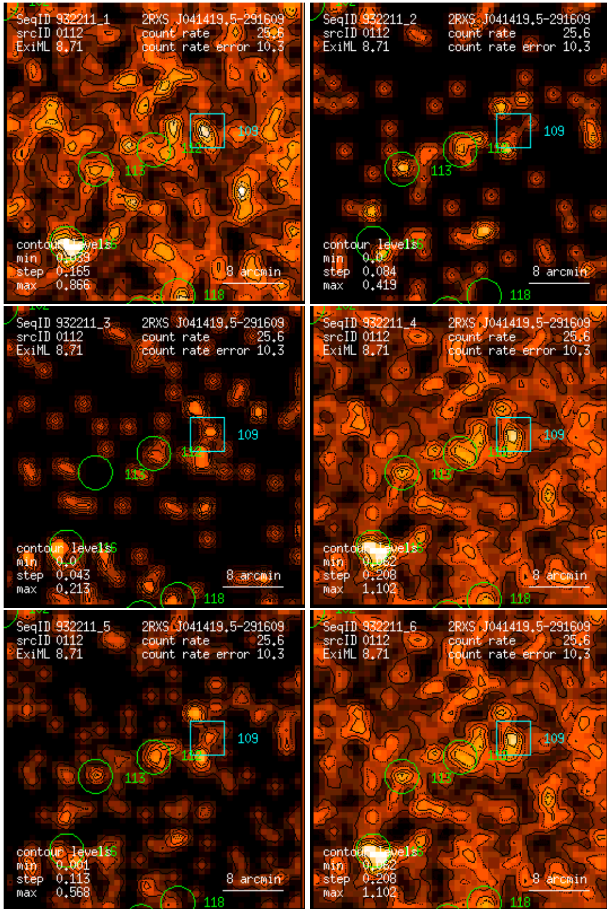
Figure 112: RASS 932211: detection 0112: band rate images, Gaussian filter: (1) PSPC channels 11 – 41, (2) 52 – 90, (3) 91 – 201, (4) 11 – 235, (5) 52 – 201, (6) 11 – 201. Broad band rates in counts/ks. Band rate contour levels in counts/ks/arcmin 2 .
