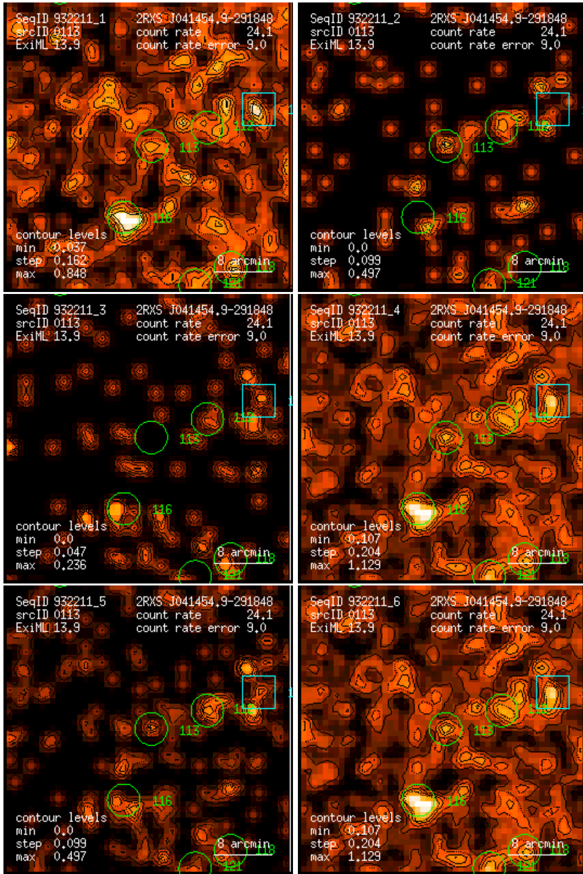
Figure 113: RASS 932211: detection 0113: band rate images, Gaussian filter: (1) PSPC channels 11 – 41, (2) 52 – 90, (3) 91 – 201, (4) 11 – 235, (5) 52 – 201, (6) 11 – 201. Broad band rates in counts/ks. Band rate contour levels in counts/ks/arcmin 2 .
