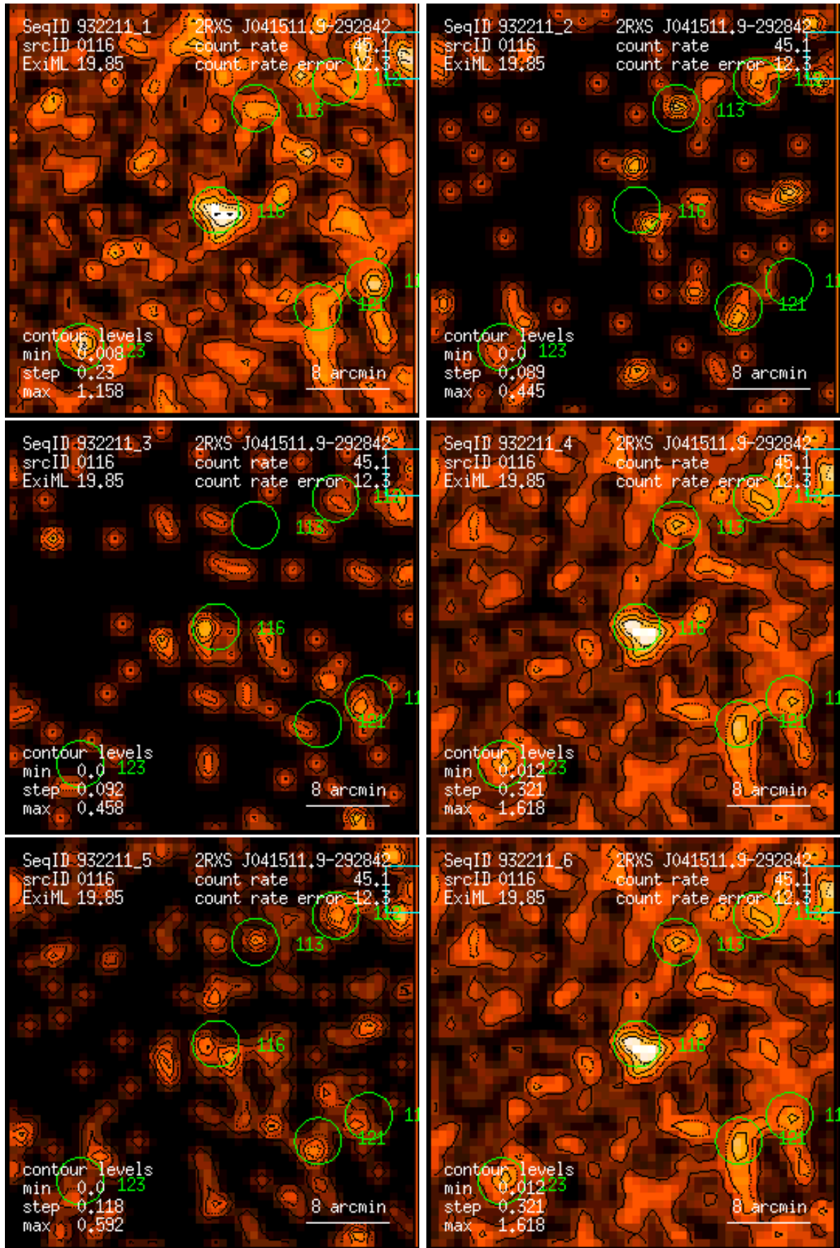
Figure 116: RASS 932211: detection 0116: band rate images, Gaussian filter: (1) PSPC channels 11 – 41, (2) 52 – 90, (3) 91 – 201, (4) 11 – 235, (5) 52 – 201, (6) 11 – 201. Broad band rates in counts/ks. Band rate contour levels in counts/ks/arcmin 2 .
