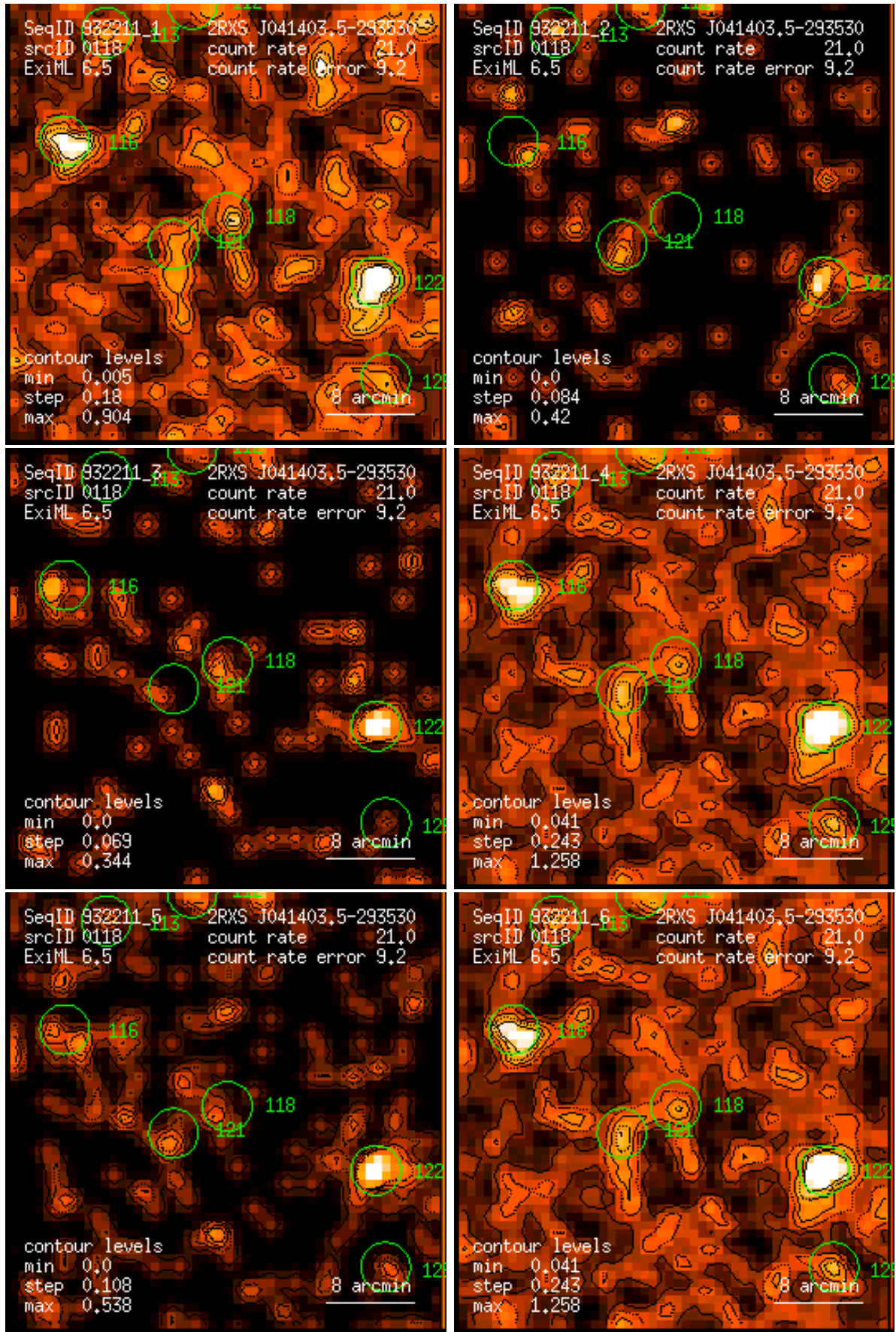
Figure 118: RASS 932211: detection 0118: band rate images, Gaussian filter: (1) PSPC channels 11 – 41, (2) 52 – 90, (3) 91 – 201, (4) 11 – 235, (5) 52 – 201, (6) 11 – 201. Broad band rates in counts/ks. Band rate contour levels in counts/ks/arcmin 2 .
