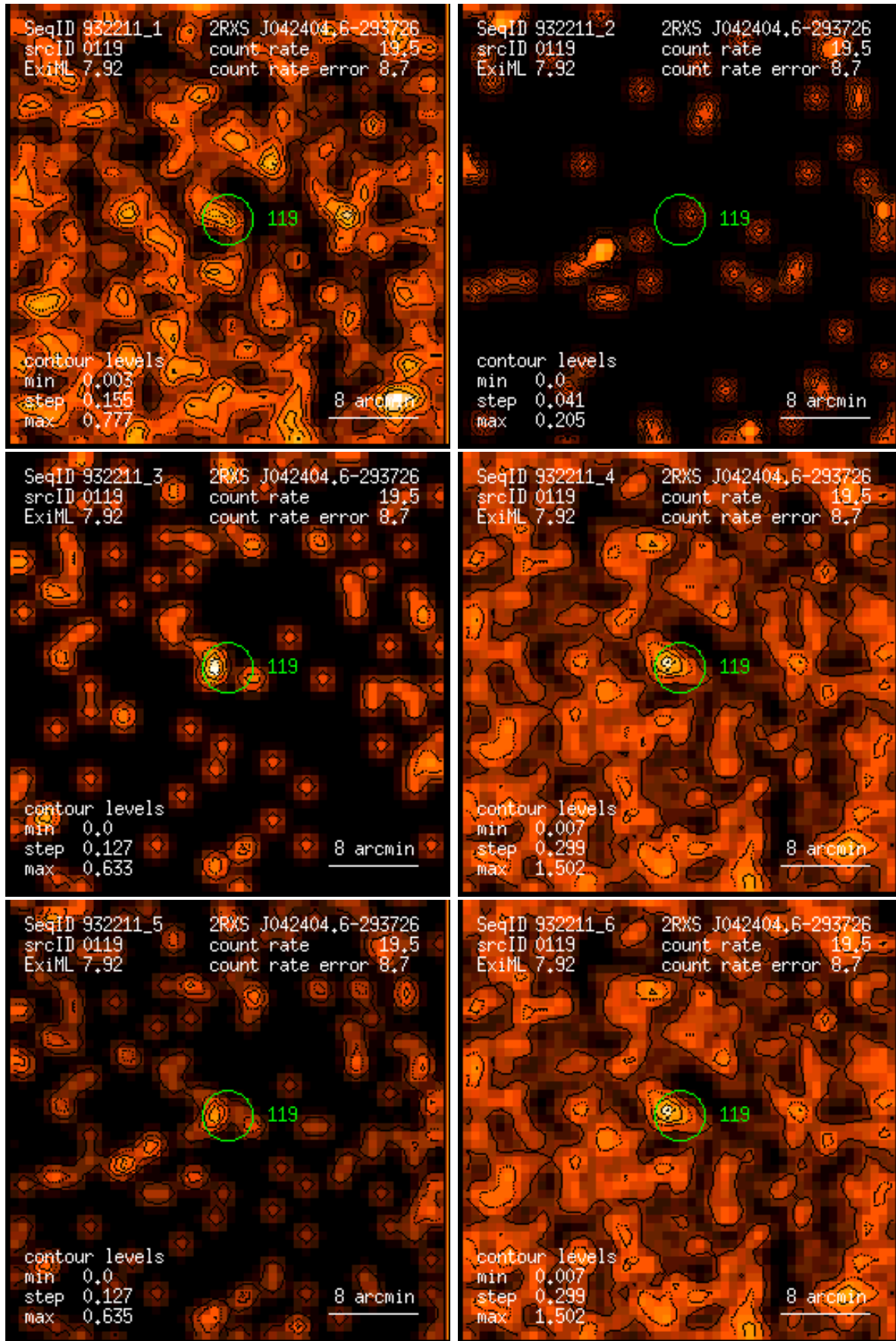
Figure 119: RASS 932211: detection 0119: band rate images, Gaussian filter: (1) PSPC channels 11 – 41, (2) 52 – 90, (3) 91 – 201, (4) 11 – 235, (5) 52 – 201, (6) 11 – 201. Broad band rates in counts/ks. Band rate contour levels in counts/ks/arcmin 2 .
