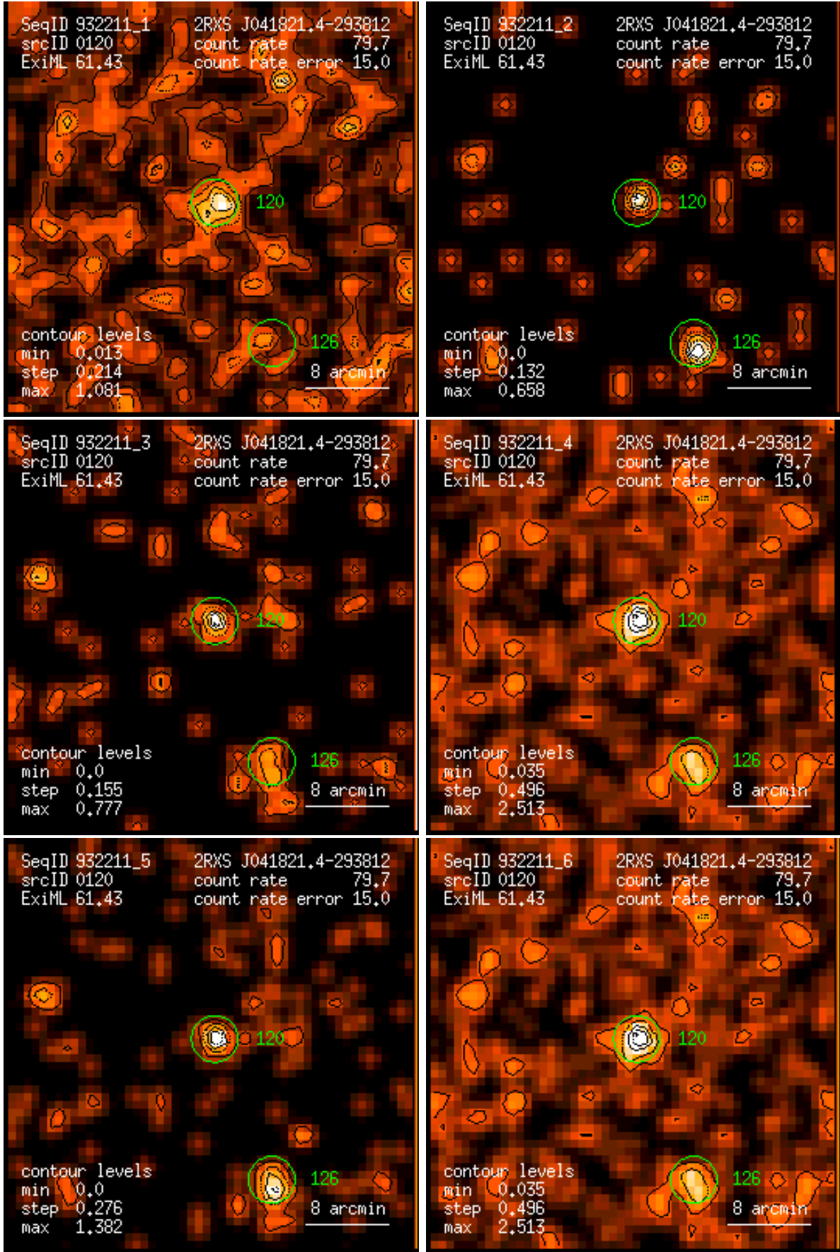
Figure 120: RASS 932211: detection 0120: band rate images, Gaussian filter: (1) PSPC channels 11 – 41, (2) 52 – 90, (3) 91 – 201, (4) 11 – 235, (5) 52 – 201, (6) 11 – 201. Broad band rates in counts/ks. Band rate contour levels in counts/ks/arcmin 2 .
