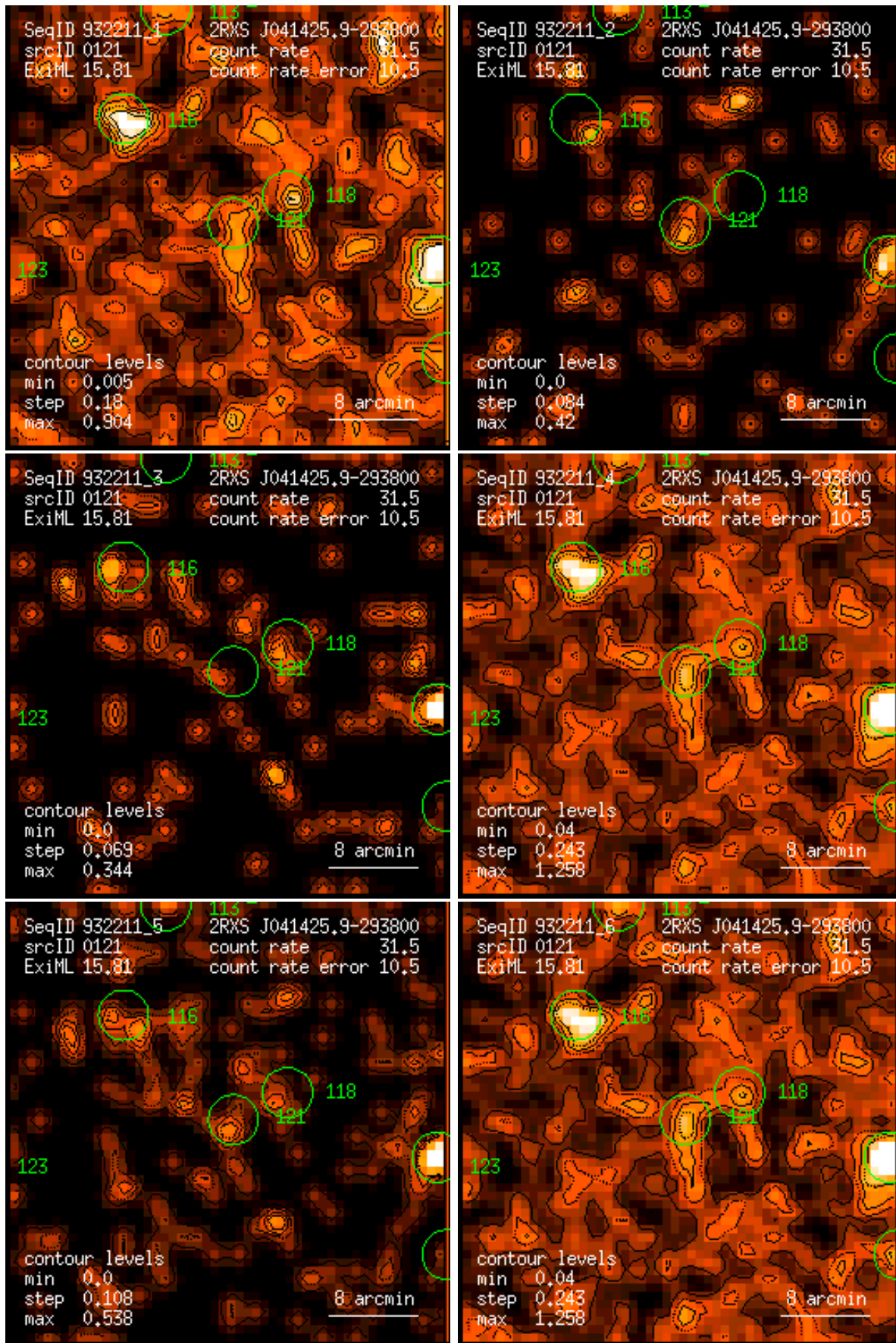
Figure 121: RASS 932211: detection 0121: band rate images, Gaussian filter: (1) PSPC channels 11 – 41, (2) 52 – 90, (3) 91 – 201, (4) 11 – 235, (5) 52 – 201, (6) 11 – 201. Broad band rates in counts/ks. Band rate contour levels in counts/ks/arcmin 2 .
