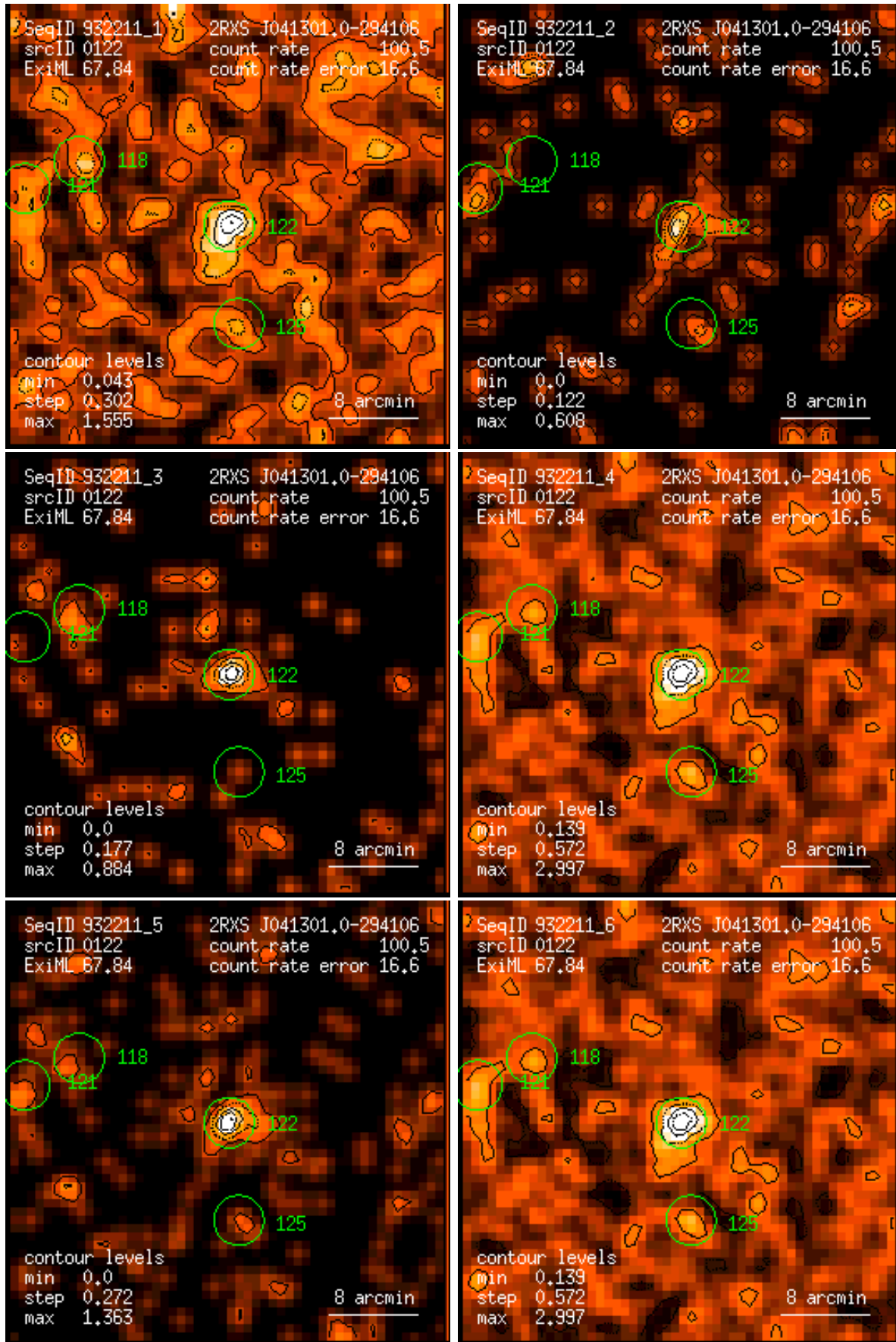
Figure 122: RASS 932211: detection 0122: band rate images, Gaussian filter: (1) PSPC channels 11 – 41, (2) 52 – 90, (3) 91 – 201, (4) 11 – 235, (5) 52 – 201, (6) 11 – 201. Broad band rates in counts/ks. Band rate contour levels in counts/ks/arcmin 2 .
