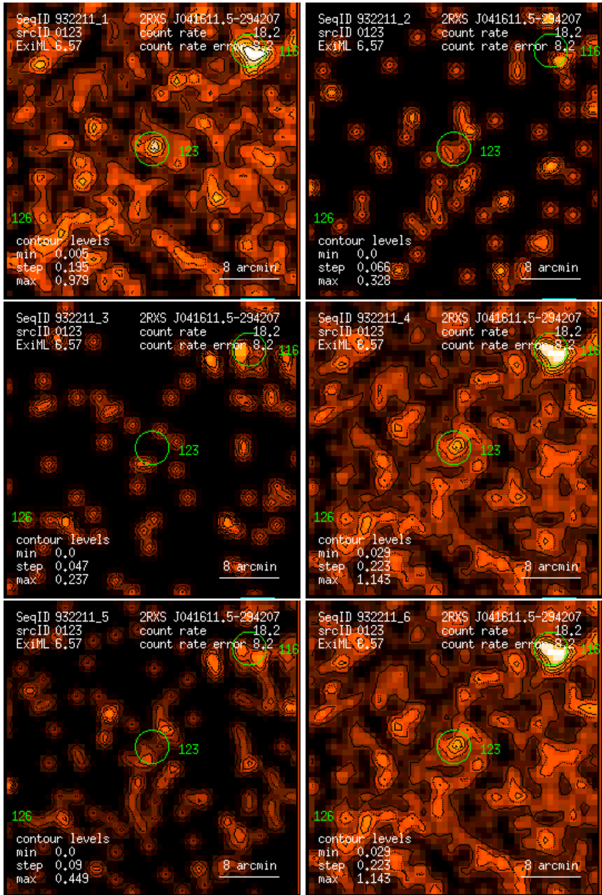
Figure 123: RASS 932211: detection 0123: band rate images, Gaussian filter: (1) PSPC channels 11 – 41, (2) 52 – 90, (3) 91 – 201, (4) 11 – 235, (5) 52 – 201, (6) 11 – 201. Broad band rates in counts/ks. Band rate contour levels in counts/ks/arcmin 2 .
