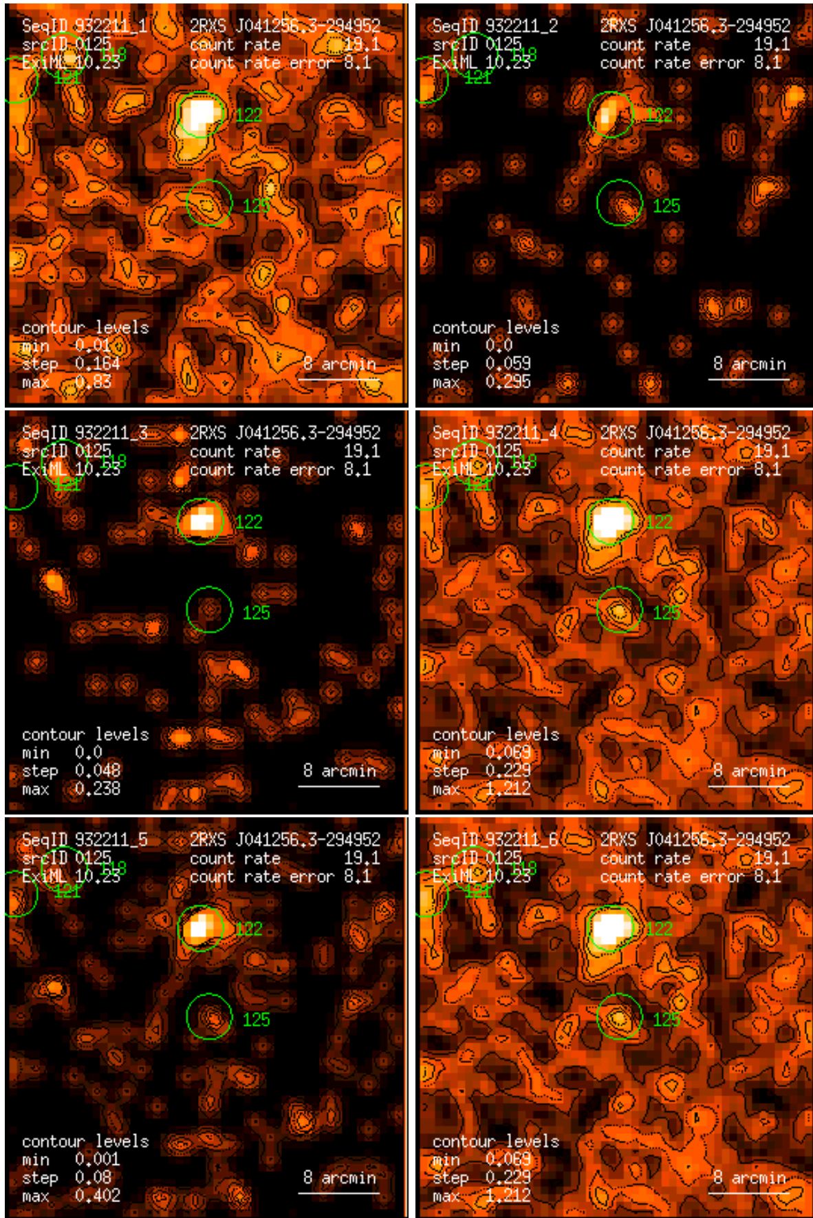
Figure 125: RASS 932211: detection 0125: band rate images, Gaussian filter: (1) PSPC channels 11 – 41, (2) 52 – 90, (3) 91 – 201, (4) 11 – 235, (5) 52 – 201, (6) 11 – 201. Broad band rates in counts/ks. Band rate contour levels in counts/ks/arcmin 2 .
