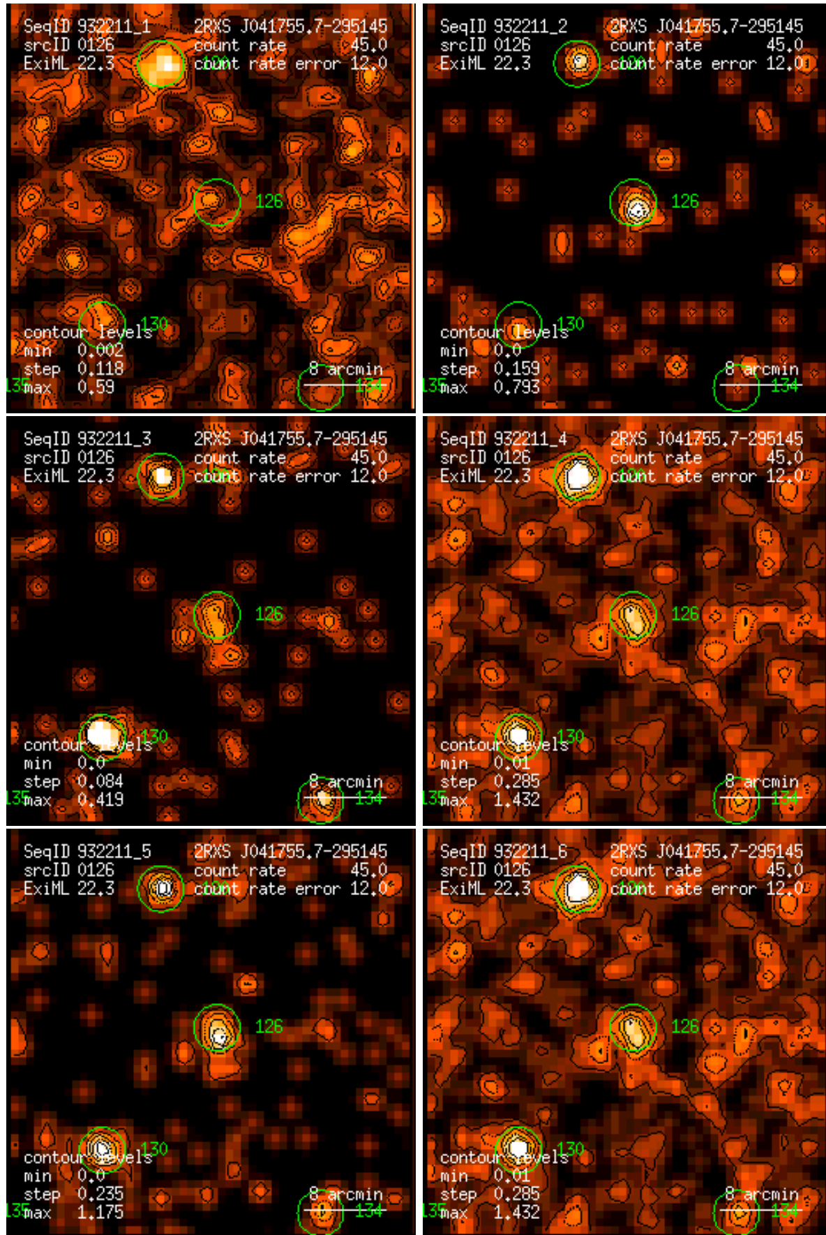
Figure 126: RASS 932211: detection 0126: band rate images, Gaussian filter: (1) PSPC channels 11 – 41, (2) 52 – 90, (3) 91 – 201, (4) 11 – 235, (5) 52 – 201, (6) 11 – 201. Broad band rates in counts/ks. Band rate contour levels in counts/ks/arcmin 2 .
