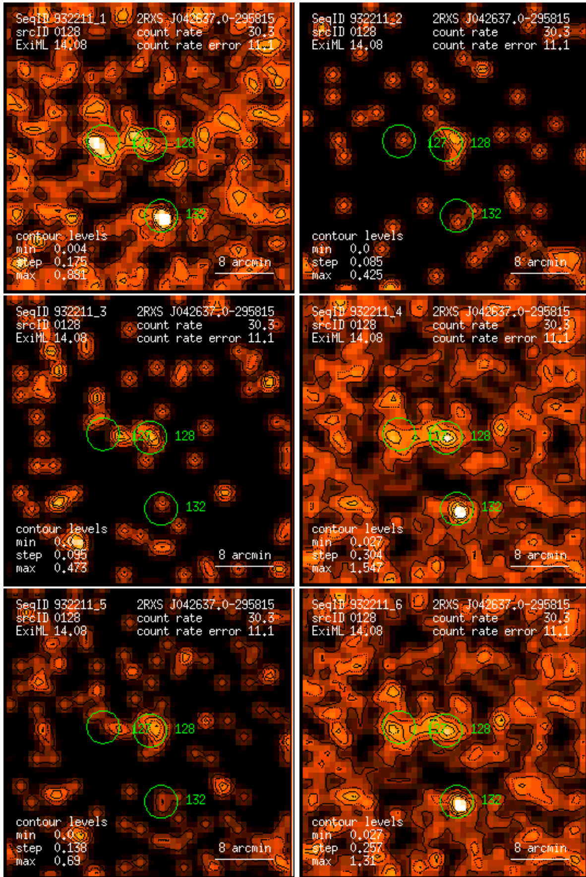
Figure 128: RASS 932211: detection 0128: band rate images, Gaussian filter: (1) PSPC channels 11 – 41, (2) 52 – 90, (3) 91 – 201, (4) 11 – 235, (5) 52 – 201, (6) 11 – 201. Broad band rates in counts/ks. Band rate contour levels in counts/ks/arcmin 2 .
