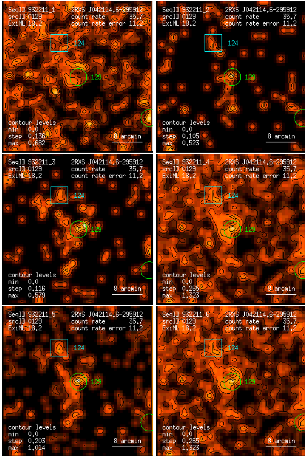
Figure 129: RASS 932211: detection 0129: band rate images, Gaussian filter: (1) PSPC channels 11 – 41, (2) 52 – 90, (3) 91 – 201, (4) 11 – 235, (5) 52 – 201, (6) 11 – 201. Broad band rates in counts/ks. Band rate contour levels in counts/ks/arcmin 2 .
