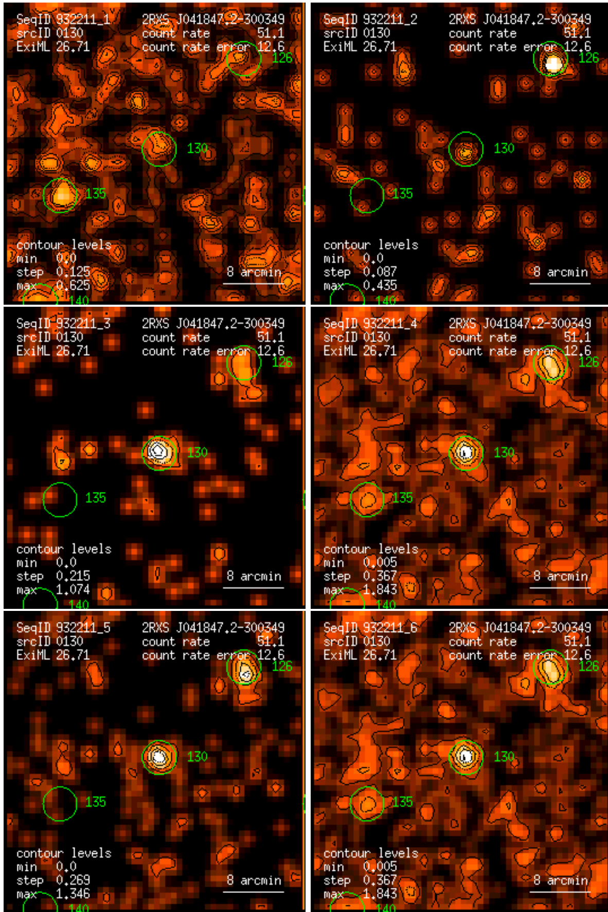
Figure 130: RASS 932211: detection 0130: band rate images, Gaussian filter: (1) PSPC channels 11 – 41, (2) 52 – 90, (3) 91 – 201, (4) 11 – 235, (5) 52 – 201, (6) 11 – 201. Broad band rates in counts/ks. Band rate contour levels in counts/ks/arcmin 2 .
