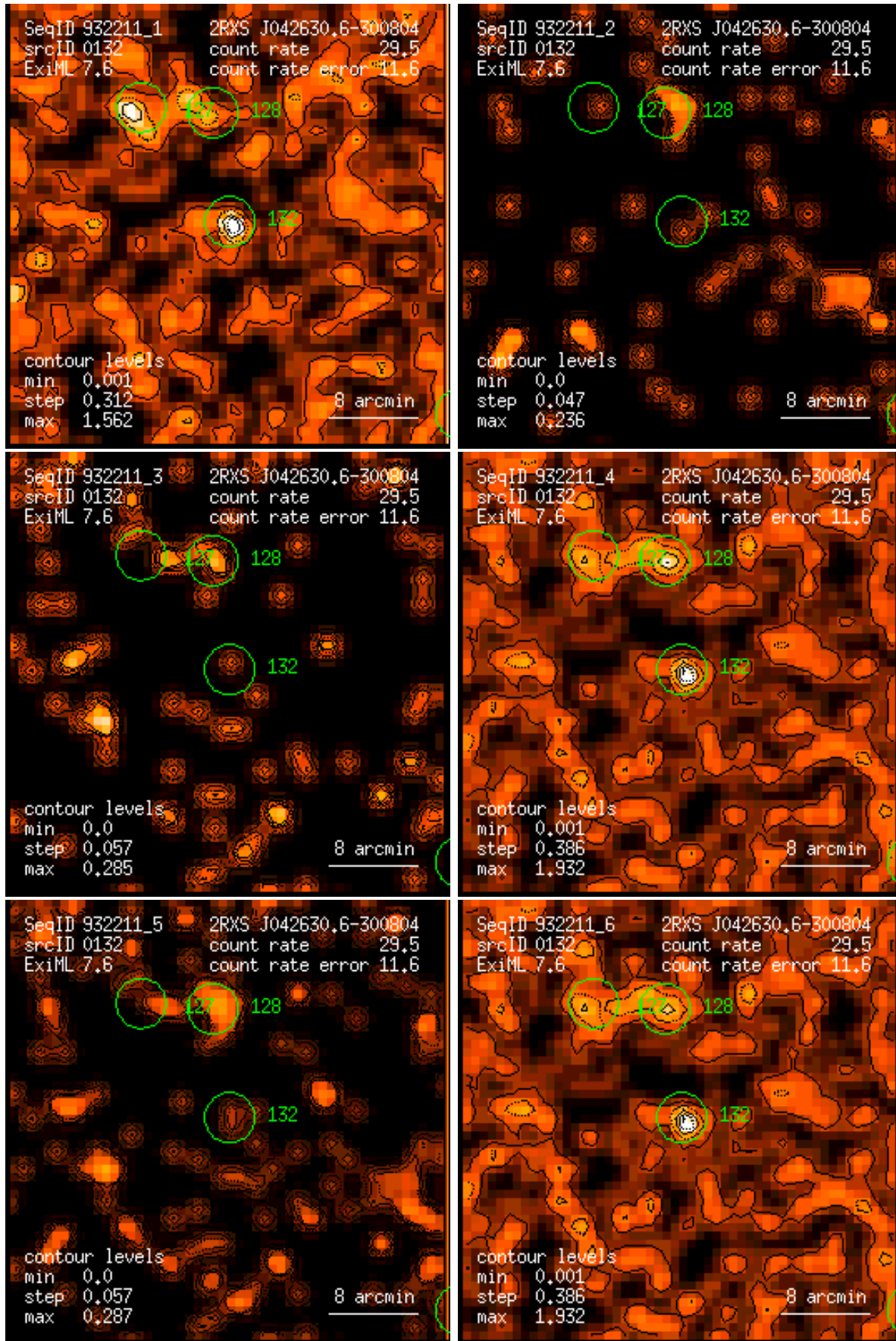
Figure 132: RASS 932211: detection 0132: band rate images, Gaussian filter: (1) PSPC channels 11 – 41, (2) 52 – 90, (3) 91 – 201, (4) 11 – 235, (5) 52 – 201, (6) 11 – 201. Broad band rates in counts/ks. Band rate contour levels in counts/ks/arcmin 2 .
