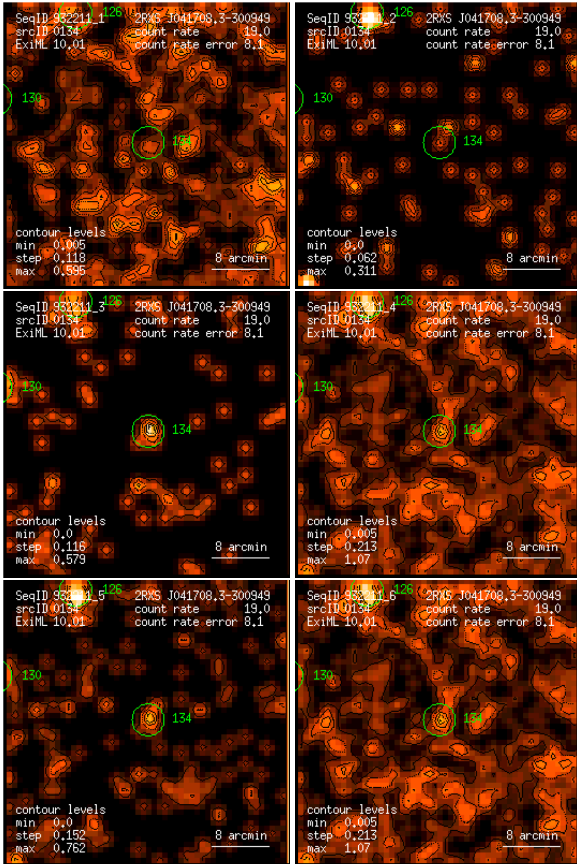
Figure 134: RASS 932211: detection 0134: band rate images, Gaussian filter: (1) PSPC channels 11 – 41, (2) 52 – 90, (3) 91 – 201, (4) 11 – 235, (5) 52 – 201, (6) 11 – 201. Broad band rates in counts/ks. Band rate contour levels in counts/ks/arcmin 2 .
