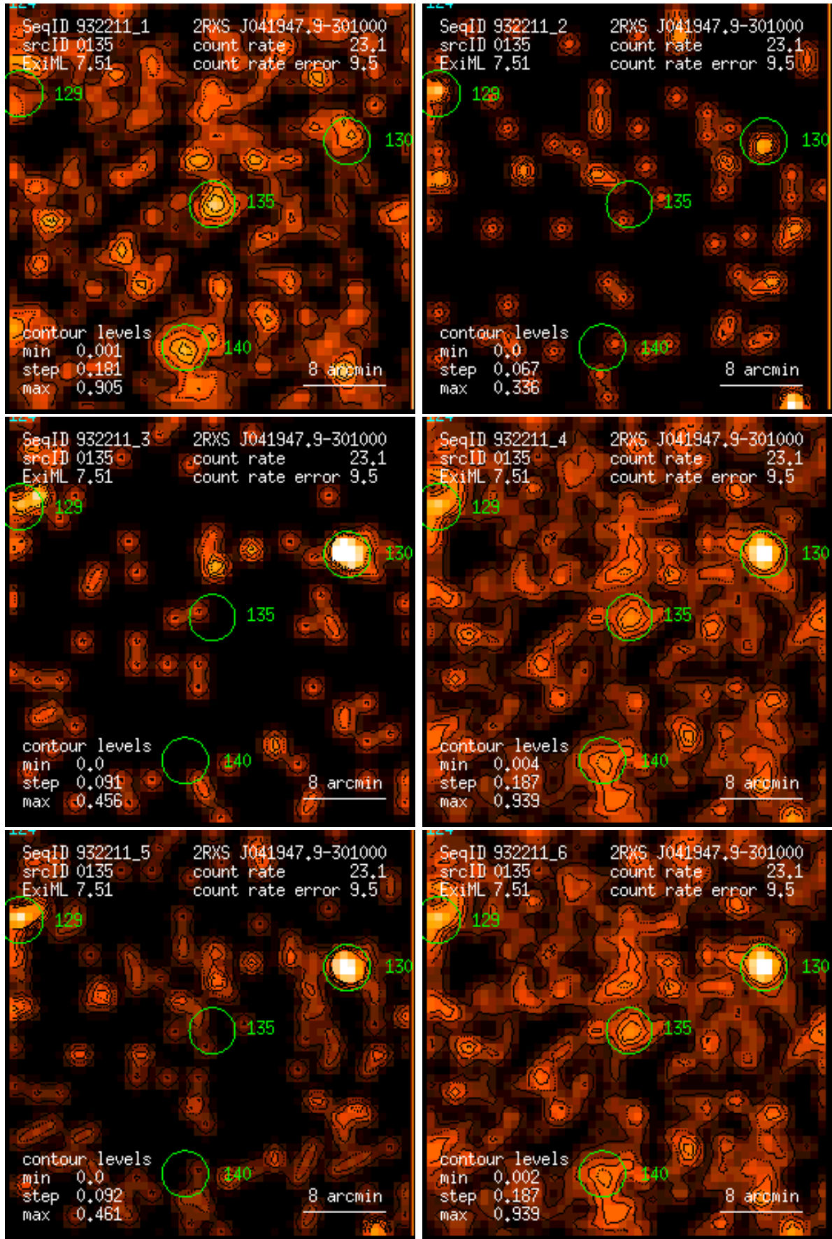
Figure 135: RASS 932211: detection 0135: band rate images, Gaussian filter: (1) PSPC channels 11 – 41, (2) 52 – 90, (3) 91 – 201, (4) 11 – 235, (5) 52 – 201, (6) 11 – 201. Broad band rates in counts/ks. Band rate contour levels in counts/ks/arcmin 2 .
