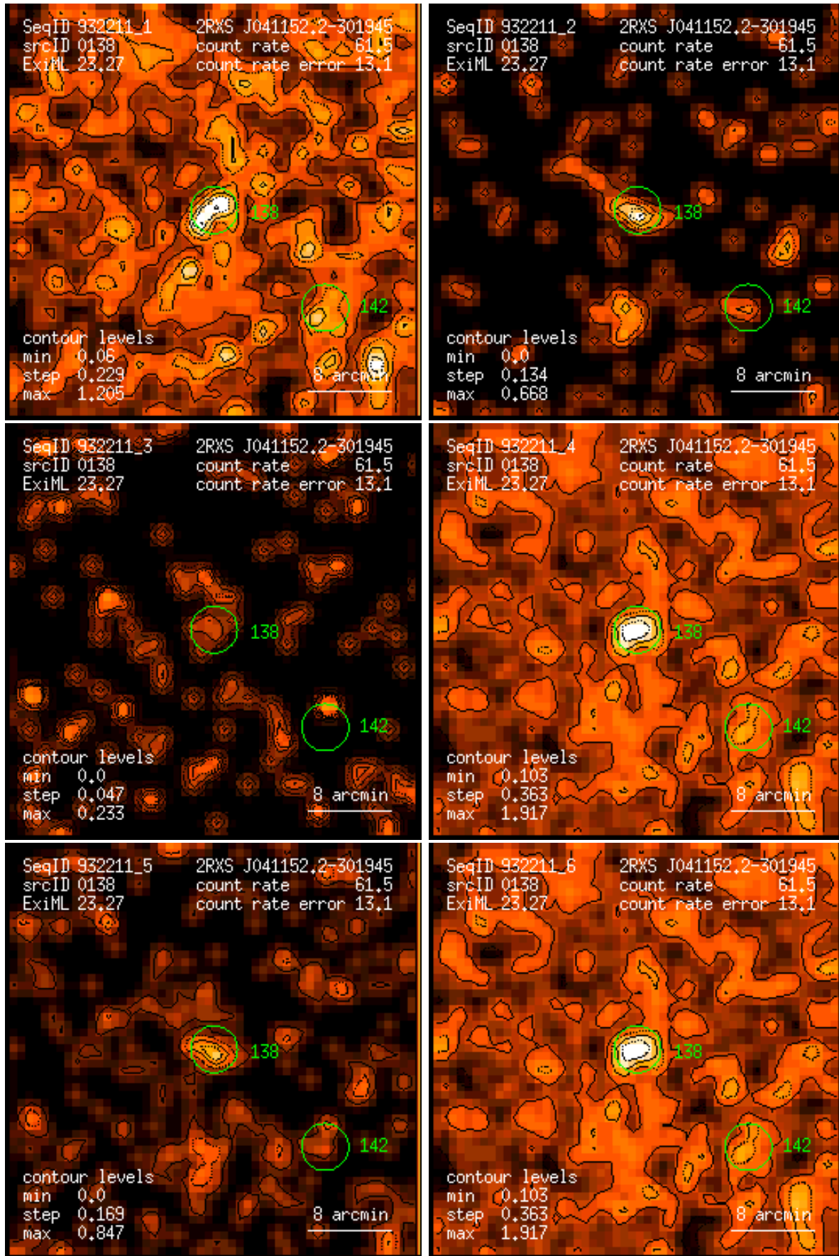
Figure 138: RASS 932211: detection 0138: band rate images, Gaussian filter: (1) PSPC channels 11 – 41, (2) 52 – 90, (3) 91 – 201, (4) 11 – 235, (5) 52 – 201, (6) 11 – 201. Broad band rates in counts/ks. Band rate contour levels in counts/ks/arcmin 2 .
